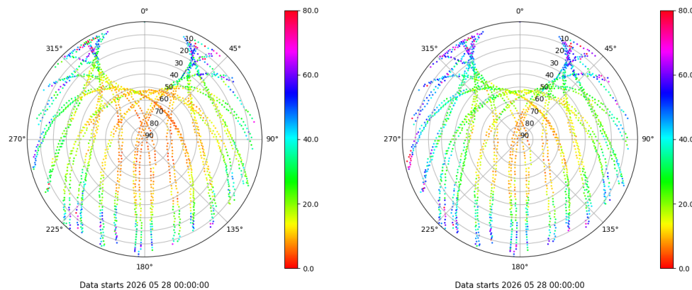
Skyplot for station HUE1. Parameter M1C Data file HUE100ESP_R_2026148.xtr Skyplot for station HUE1. Parameter M2P Data file HUE100ESP_R_2026148.xtr
