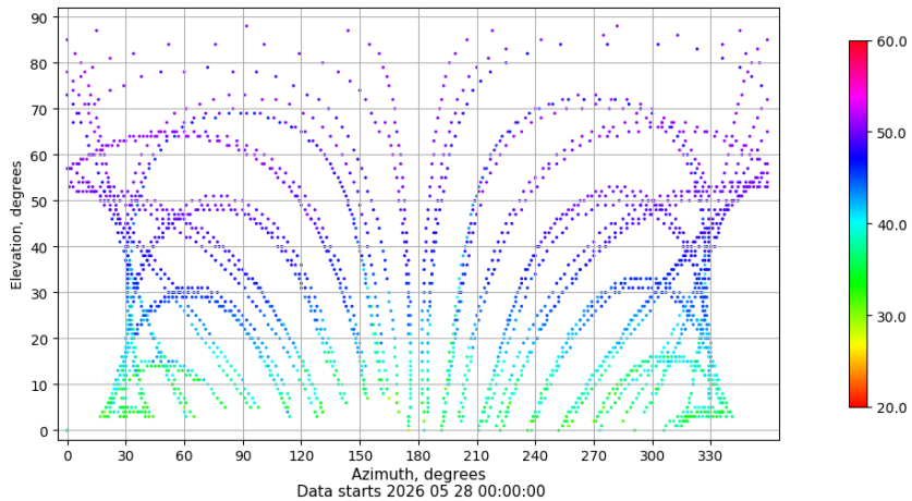
Azimuth-elevation plot for station HUE1. Signal to Noise S1C Data file HUE100ESP_R_2026148.xtr
