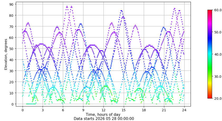
Time-elevation plot for station HUE1. Signal to Noise S1C Data file HUE100ESP_R_2026148.xtr
