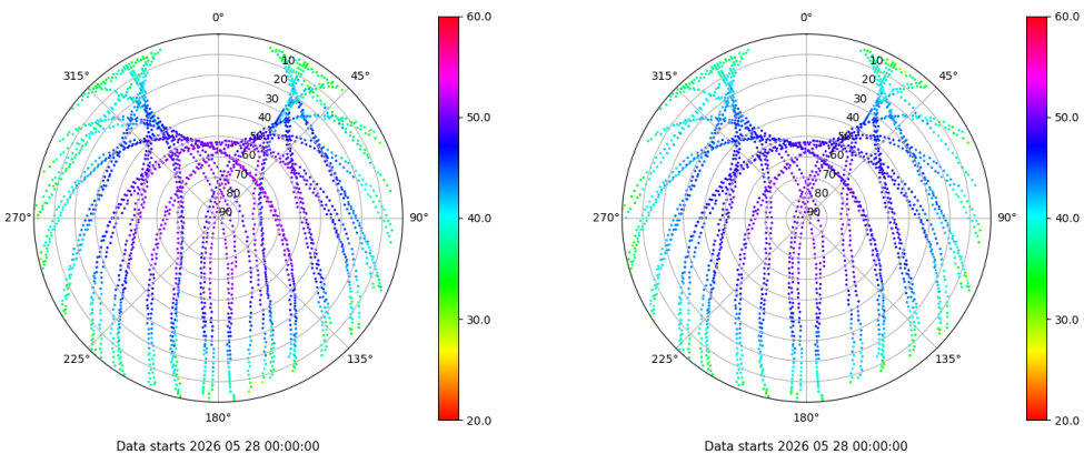
Skyplot for station HUE1. Signal to Noise S1C Data file HUE100ESP_R_2026148.xtr Skyplot for station HUE1. Signal to Noise S2P Data file HUE100ESP_R_2026148.xtr
