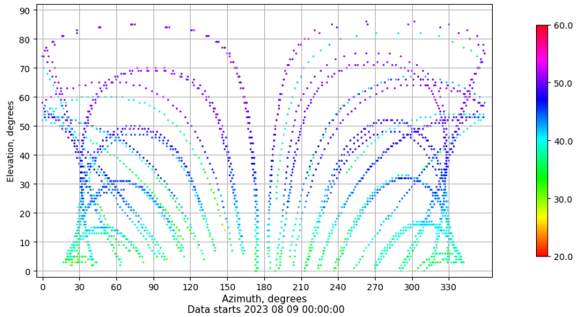
Azimuth-elevation plot for station HUE1. Signal to Noise S1C Data file HUE100ESP_R_2023221.xtr
