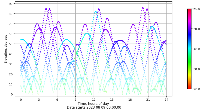
Time-elevation plot for station HUE1. Signal to Noise S1C Data file HUE100ESP_R_2023221.xtr
