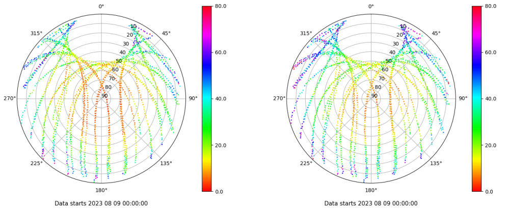
Skyplot for station HUE1. Parameter M1C Data file HUE100ESP_R_2023221.xtr Skyplot for station HUE1. Parameter M2P Data file HUE100ESP_R_2023221.xtr
