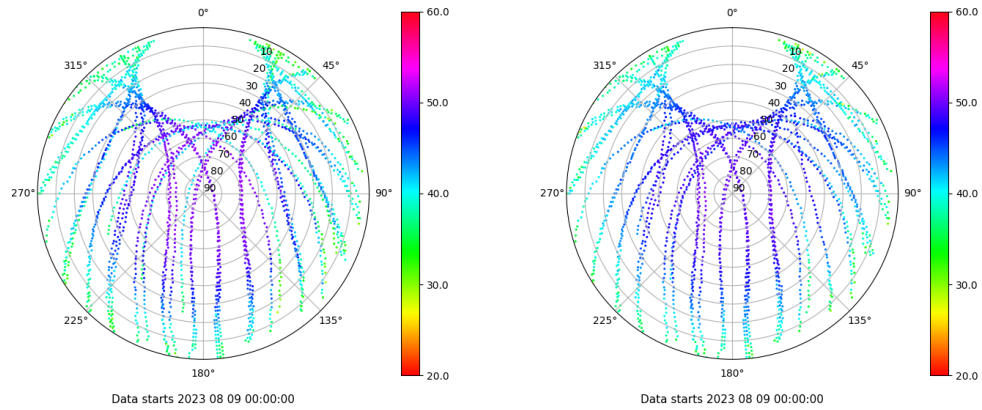
Skyplot for station HUE1. Signal to Noise S1C Data file HUE100ESP_R_2023221.xtr Skyplot for station HUE1. Signal to Noise S2P Data file HUE100ESP_R_2023221.xtr
