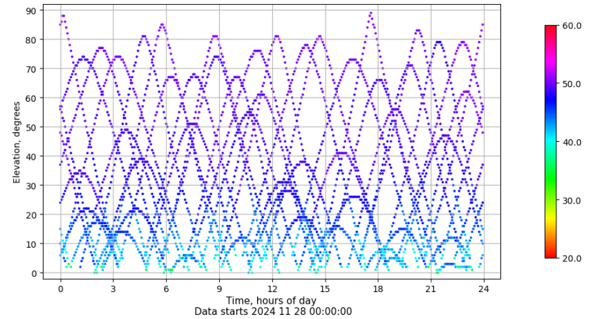
Time-elevation plot for station GIRO. Signal to Noise S1C Data file GIRO00ESP_R_2024333.xtr
