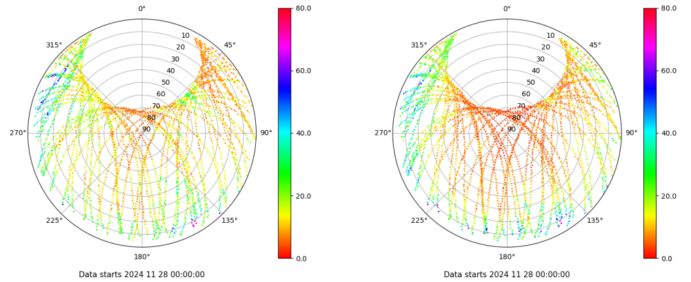
Skyplot for station GIRO. Parameter M1C Data file GIRO00ESP_R_2024333.xtr Skyplot for station GIRO. Parameter M2W Data file GIRO00ESP_R_2024333.xtr
