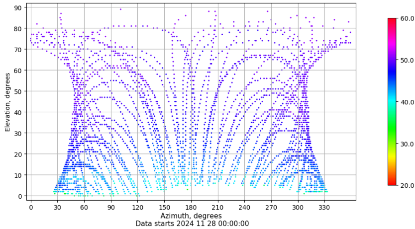
Azimuth-elevation plot for station GIRO. Signal to Noise S1C Data file GIRO00ESP_R_2024333.xtr
