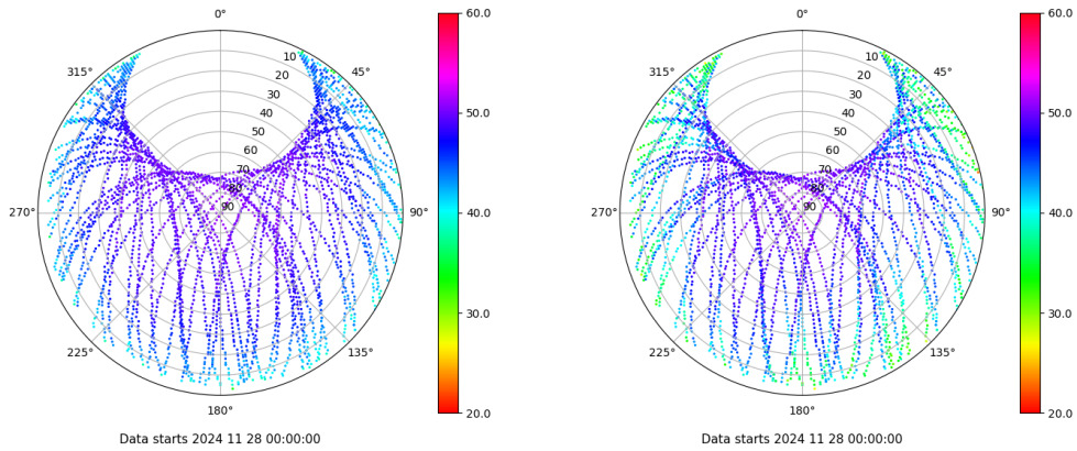
Skyplot for station GIRO. Signal to Noise S1C Data file GIRO00ESP_R_2024333.xtr Skyplot for station GIRO. Signal to Noise S2W Data file GIRO00ESP_R_2024333.xtr
