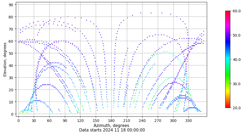
Azimuth-elevation plot for station GIRO. Signal to Noise S1C Data file GIRO00ESP_R_2024323.xtr
