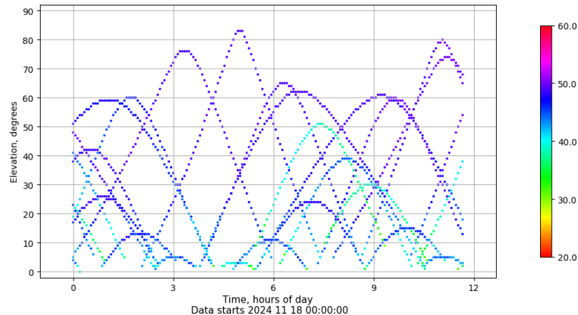
Time-elevation plot for station GIRO. Signal to Noise S1C Data file GIRO00ESP_R_2024323.xtr
