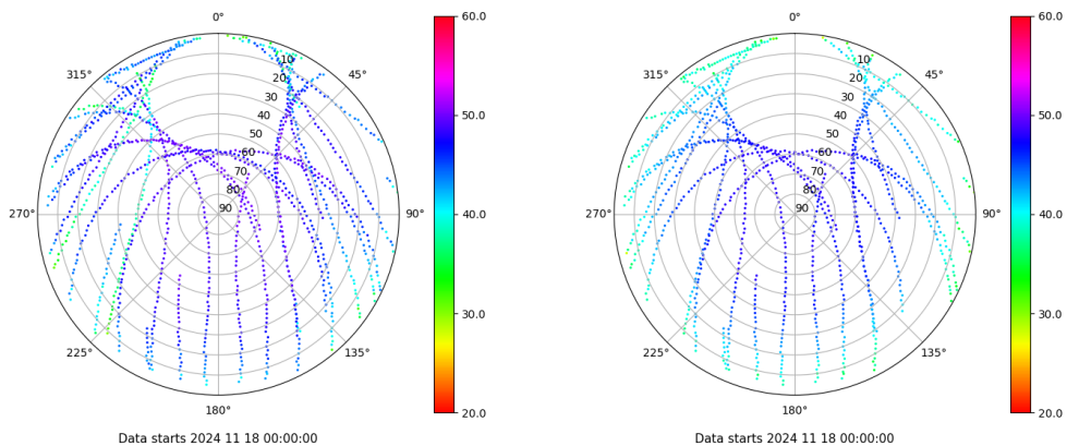
Skyplot for station GIRO. Signal to Noise S1C Data file GIRO00ESP_R_2024323.xtr Skyplot for station GIRO. Signal to Noise S2P Data file GIRO00ESP_R_2024323.xtr
