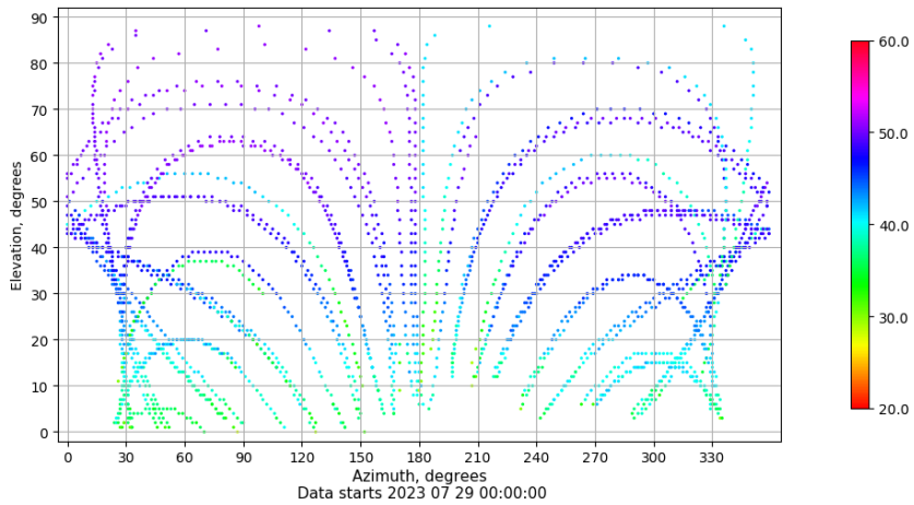
Azimuth-elevation plot for station FUER. Signal to Noise S1C Data file FUER00ESP_R_2023210.xtr
