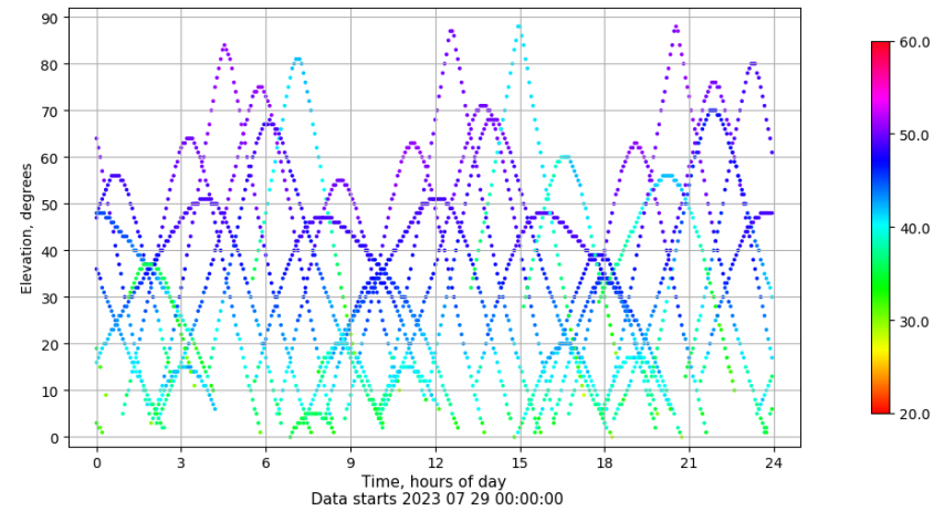
Time-elevation plot for station FUER. Signal to Noise S1C Data file FUER00ESP_R_2023210.xtr
