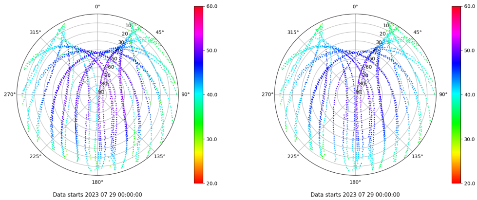
Skyplot for station FUER. Signal to Noise S1C Data file FUER00ESP_R_2023210.xtr Skyplot for station FUER. Signal to Noise S2P Data file FUER00ESP_R_2023210.xtr
