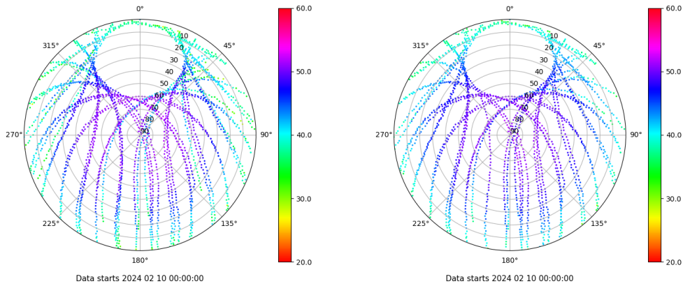
Skyplot for station FRRL. Signal to Noise S1C Data file FRRL00ESP_R_2024041.xtr Skyplot for station FRRL. Signal to Noise S2P Data file FRRL00ESP_R_2024041.xtr
