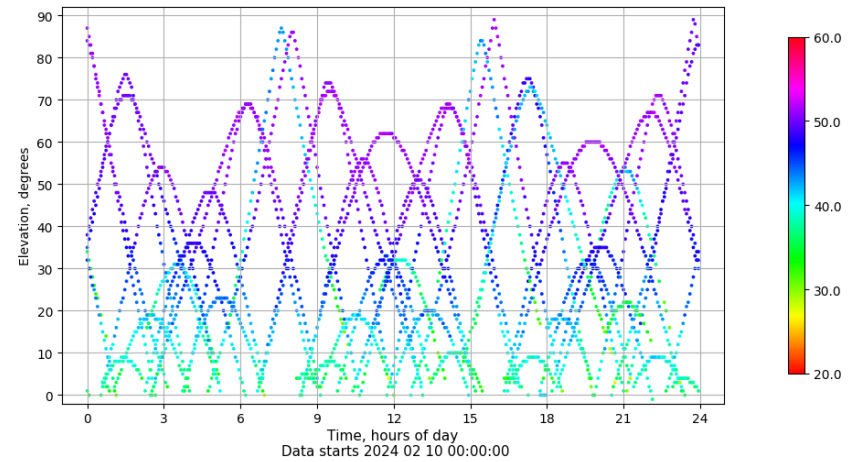
Time-elevation plot for station FRRL. Signal to Noise S1C Data file FRRL00ESP_R_2024041.xtr
