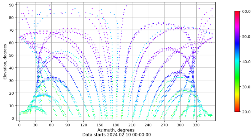
Azimuth-elevation plot for station FRRL. Signal to Noise S1C Data file FRRL00ESP_R_2024041.xtr
