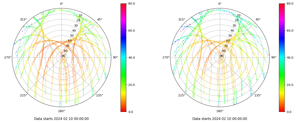
Skyplot for station FRRL. Parameter M1C Data file FRRL00ESP_R_2024041.xtr Skyplot for station FRRL. Parameter M2P Data file FRRL00ESP_R_2024041.xtr
