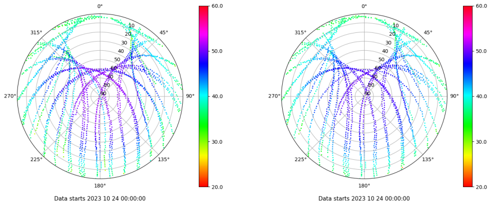
Skyplot for station FRRL. Signal to Noise S1C Data file FRRL00ESP_R_2023297.xtr Skyplot for station FRRL. Signal to Noise S2P Data file FRRL00ESP_R_2023297.xtr
