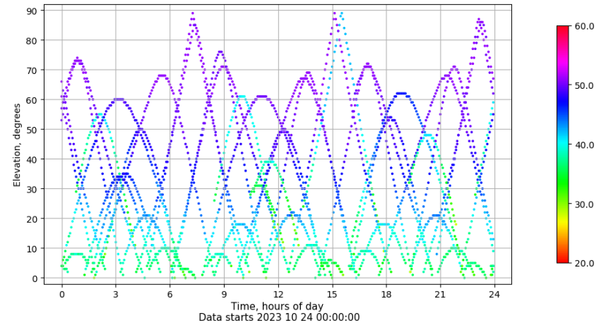
Time-elevation plot for station FRRL. Signal to Noise S1C Data file FRRL00ESP_R_2023297.xtr
