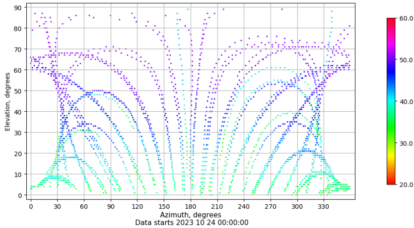
Azimuth-elevation plot for station FRRL. Signal to Noise S1C Data file FRRL00ESP_R_2023297.xtr
