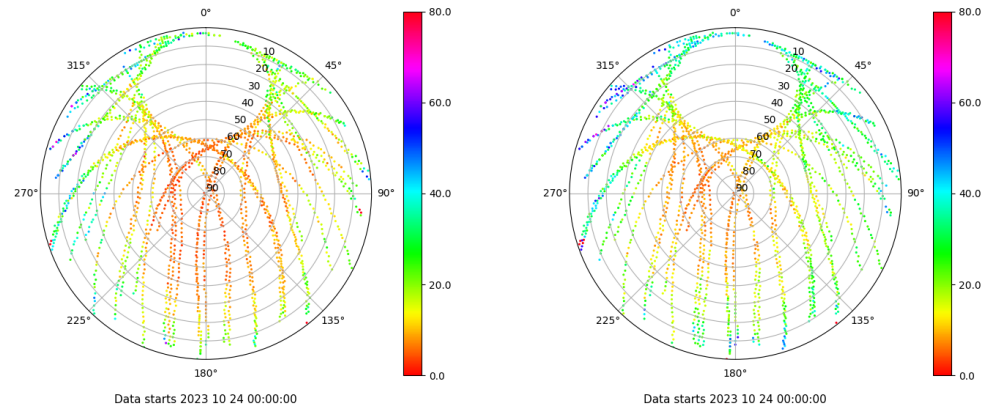
Skyplot for station FRRL. Parameter M1C Data file FRRL00ESP_R_2023297.xtr Skyplot for station FRRL. Parameter M2P Data file FRRL00ESP_R_2023297.xtr
