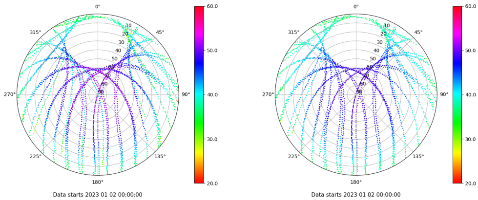
Skyplot for station FRRL. Signal to Noise S1C Data file FRRL00ESP_R_2023002.xtr Skyplot for station FRRL. Signal to Noise S2P Data file FRRL00ESP_R_2023002.xtr
