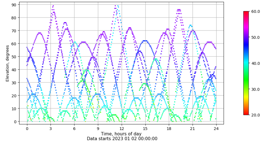
Time-elevation plot for station FRRL. Signal to Noise S1C Data file FRRL00ESP_R_2023002.xtr
