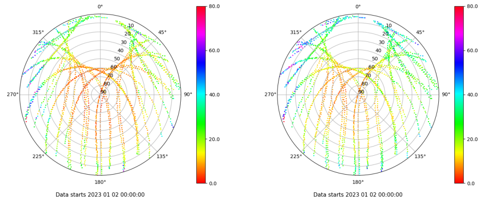
Skyplot for station FRRL. Parameter M1C Data file FRRL00ESP_R_2023002.xtr Skyplot for station FRRL. Parameter M2P Data file FRRL00ESP_R_2023002.xtr
