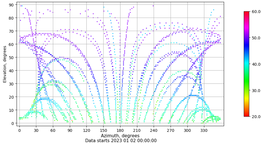
Azimuth-elevation plot for station FRRL. Signal to Noise S1C Data file FRRL00ESP_R_2023002.xtr
