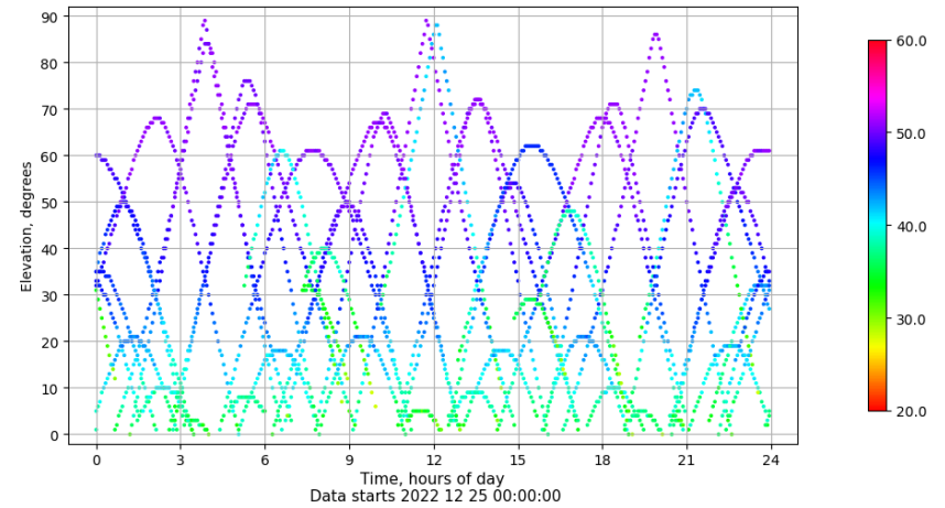
Time-elevation plot for station FRRL. Signal to Noise S1C Data file FRRL00ESP_R_2022359.xtr
