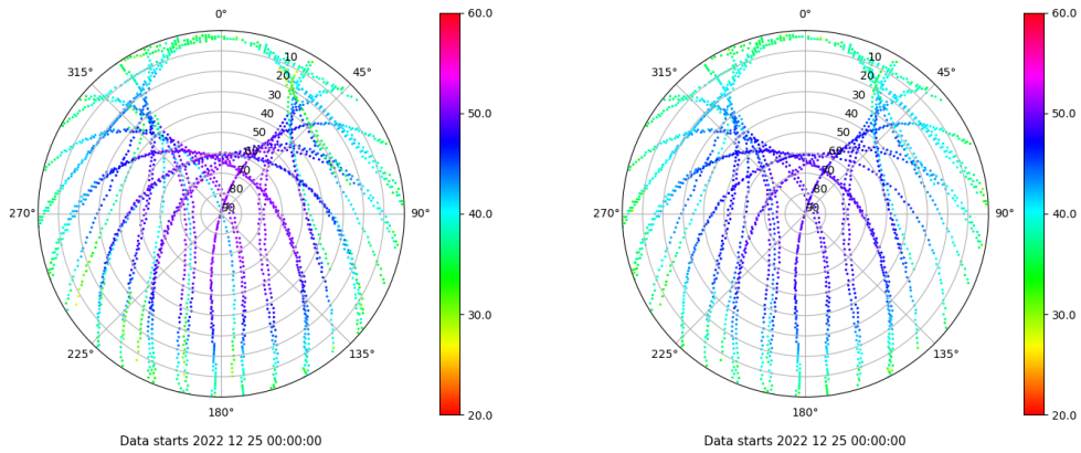
Skyplot for station FRRL. Signal to Noise S1C Data file FRRL00ESP_R_2022359.xtr Skyplot for station FRRL. Signal to Noise S2P Data file FRRL00ESP_R_2022359.xtr
