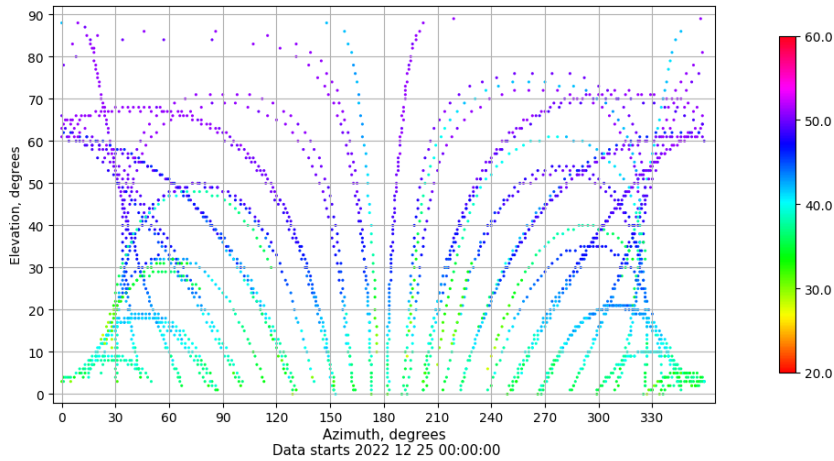
Azimuth-elevation plot for station FRRL. Signal to Noise S1C Data file FRRL00ESP_R_2022359.xtr
