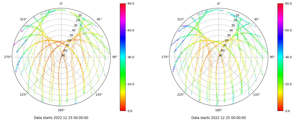
Skyplot for station FRRL. Parameter M1C Data file FRRL00ESP_R_2022359.xtr Skyplot for station FRRL. Parameter M2P Data file FRRL00ESP_R_2022359.xtr
