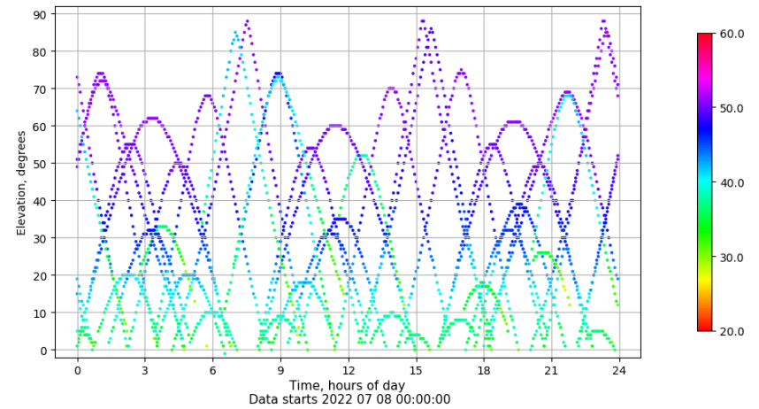
Time-elevation plot for station FRRL. Signal to Noise S1C Data file FRRL00ESP_R_2022189.xtr
