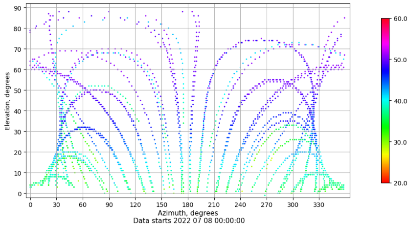
Azimuth-elevation plot for station FRRL. Signal to Noise S1C Data file FRRL00ESP_R_2022189.xtr
