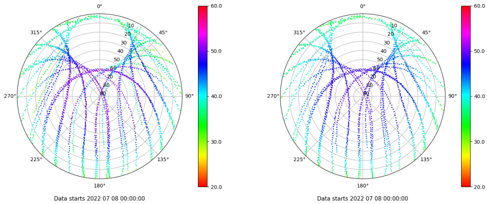
Skyplot for station FRRL. Signal to Noise S1C Data file FRRL00ESP_R_2022189.xtr Skyplot for station FRRL. Signal to Noise S2P Data file FRRL00ESP_R_2022189.xtr
