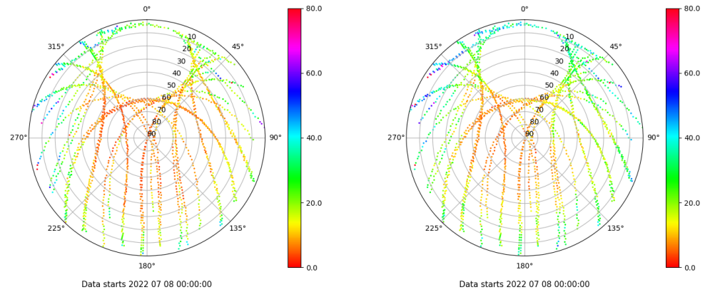
Skyplot for station FRRL. Parameter M1C Data file FRRL00ESP_R_2022189.xtr Skyplot for station FRRL. Parameter M2P Data file FRRL00ESP_R_2022189.xtr
