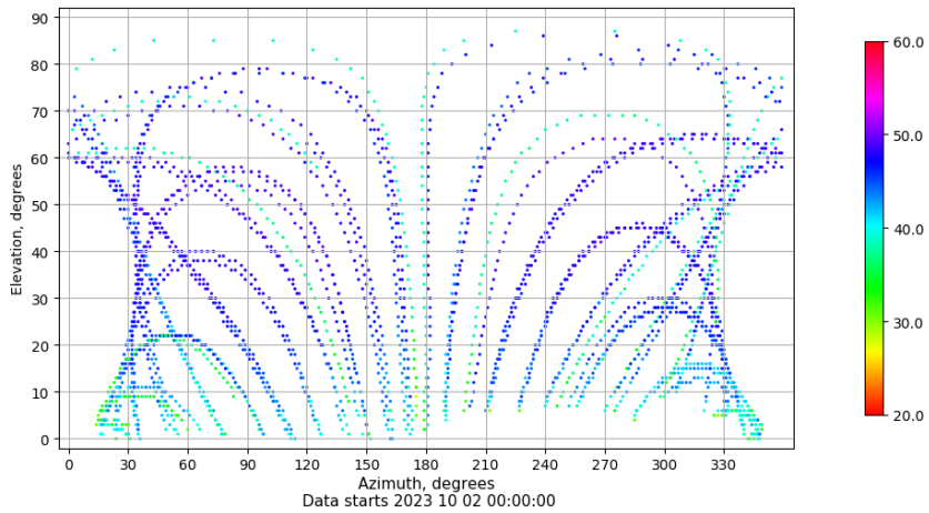
Azimuth-elevation plot for station FRAG. Signal to Noise S1C Data file FRAG00ESP_R_2023275.xtr
