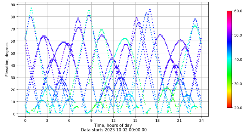
Time-elevation plot for station FRAG. Signal to Noise S1C Data file FRAG00ESP_R_2023275.xtr
