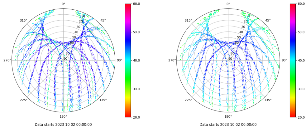
Skyplot for station FRAG. Signal to Noise S1C Data file FRAG00ESP_R_2023275.xtr Skyplot for station FRAG. Signal to Noise S2P Data file FRAG00ESP_R_2023275.xtr
