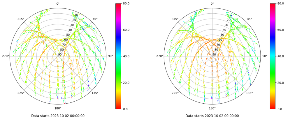
Skyplot for station FRAG. Parameter M1C Data file FRAG00ESP_R_2023275.xtr Skyplot for station FRAG. Parameter M2P Data file FRAG00ESP_R_2023275.xtr
