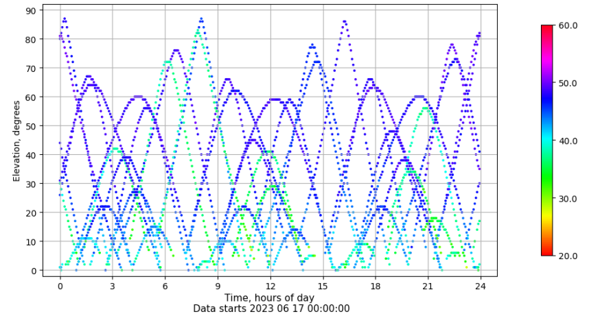
Time-elevation plot for station FRAG. Signal to Noise S1C Data file FRAG00ESP_R_2023168.xtr
