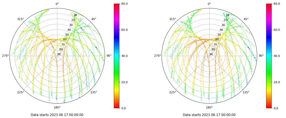
Skyplot for station FRAG. Parameter M1C Data file FRAG00ESP_R_2023168.xtr Skyplot for station FRAG. Parameter M2P Data file FRAG00ESP_R_2023168.xtr
