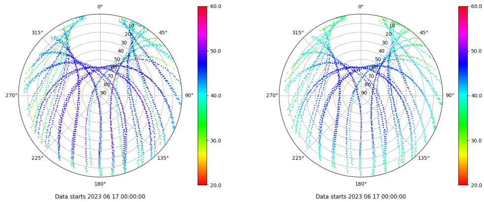
Skyplot for station FRAG. Signal to Noise S1C Data file FRAG00ESP_R_2023168.xtr Skyplot for station FRAG. Signal to Noise S2P Data file FRAG00ESP_R_2023168.xtr
