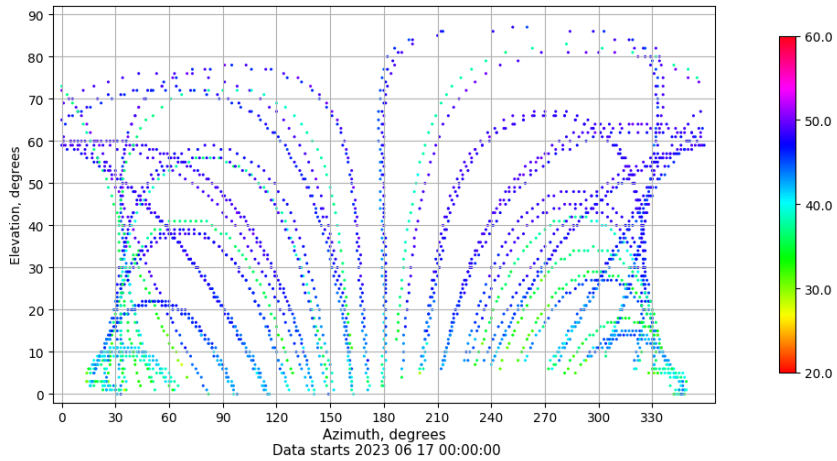
Azimuth-elevation plot for station FRAG. Signal to Noise S1C Data file FRAG00ESP_R_2023168.xtr
