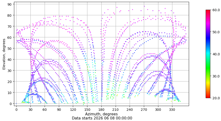
Azimuth-elevation plot for station EIVI. Signal to Noise S1C Data file EIVI00ESP_R_2026159.xtr
