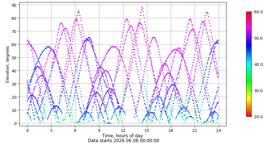
Time-elevation plot for station EIVI. Signal to Noise S1C Data file EIVI00ESP_R_2026159.xtr
