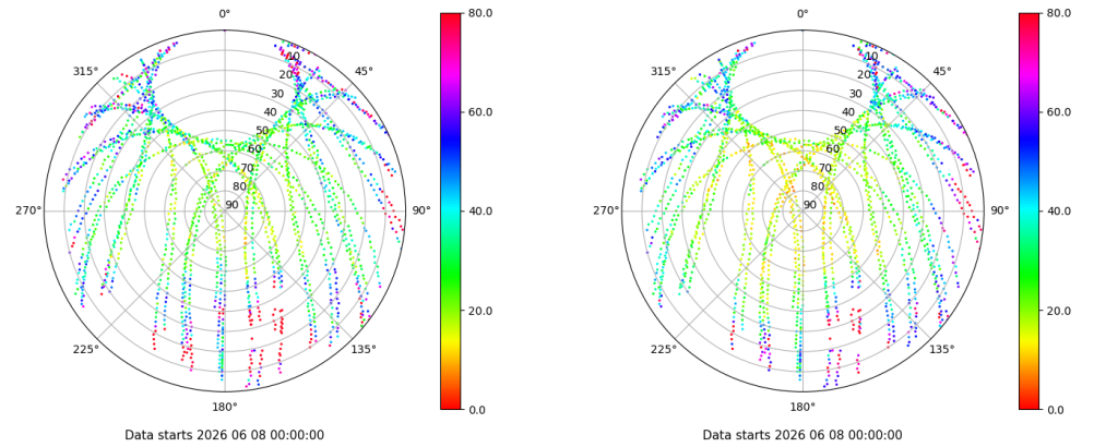
Skyplot for station EIVI. Parameter M1C Data file EIVI00ESP_R_2026159.xtr Skyplot for station EIVI. Parameter M2P Data file EIVI00ESP_R_2026159.xtr
