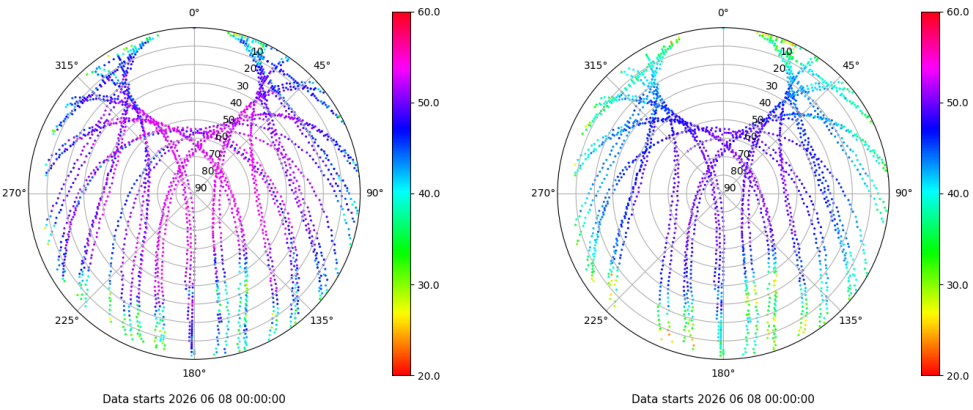
Skyplot for station EIVI. Signal to Noise S1C Data file EIVI00ESP_R_2026159.xtr Skyplot for station EIVI. Signal to Noise S2P Data file EIVI00ESP_R_2026159.xtr
