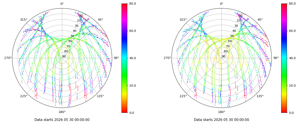
Skyplot for station EIVI. Parameter M1C Data file EIVI00ESP_R_2026150.xtr Skyplot for station EIVI. Parameter M2P Data file EIVI00ESP_R_2026150.xtr
