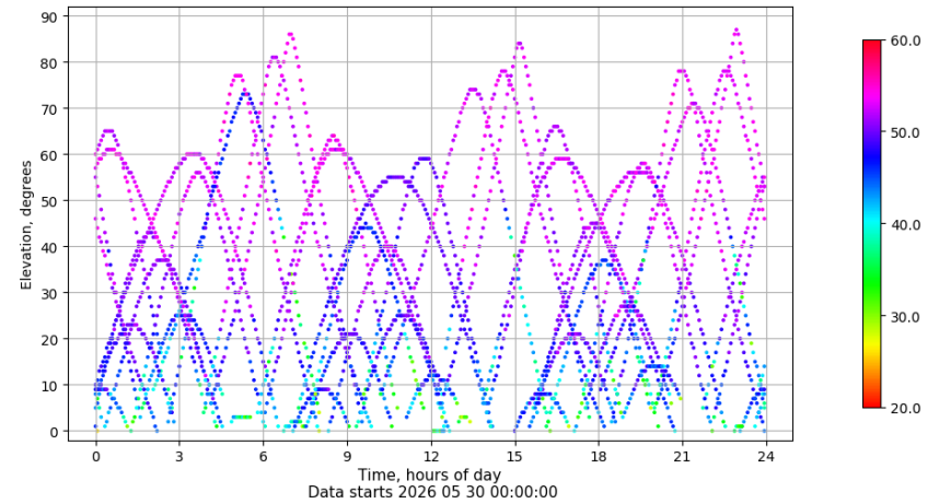
Time-elevation plot for station EIVI. Signal to Noise S1C Data file EIVI00ESP_R_2026150.xtr
