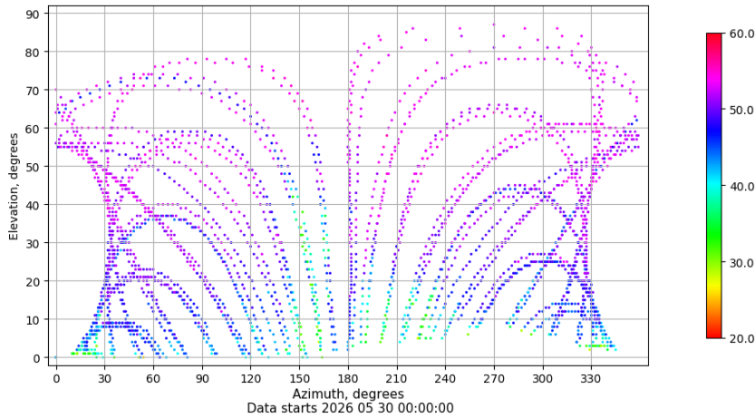
Azimuth-elevation plot for station EIVI. Signal to Noise S1C Data file EIVI00ESP_R_2026150.xtr
