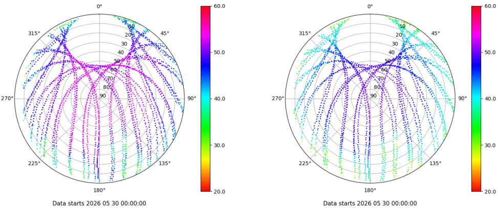
Skyplot for station EIVI. Signal to Noise S1C Data file EIVI00ESP_R_2026150.xtr Skyplot for station EIVI. Signal to Noise S2P Data file EIVI00ESP_R_2026150.xtr
