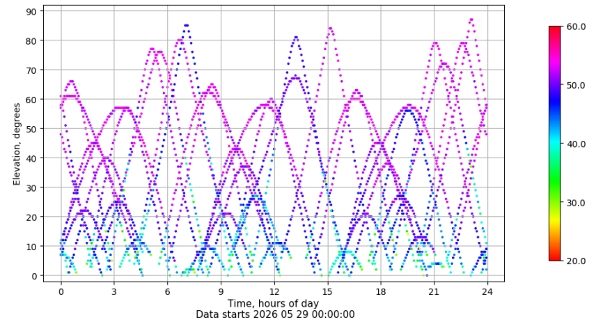
Time-elevation plot for station EIVI. Signal to Noise S1C Data file EIVI00ESP_R_2026149.xtr
