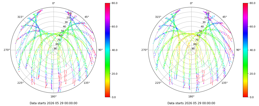
Skyplot for station EIVI. Parameter M1C Data file EIVI00ESP_R_2026149.xtr Skyplot for station EIVI. Parameter M2P Data file EIVI00ESP_R_2026149.xtr
