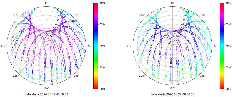
Skyplot for station EIVI. Signal to Noise S1C Data file EIVI00ESP_R_2026149.xtr Skyplot for station EIVI. Signal to Noise S2P Data file EIVI00ESP_R_2026149.xtr
