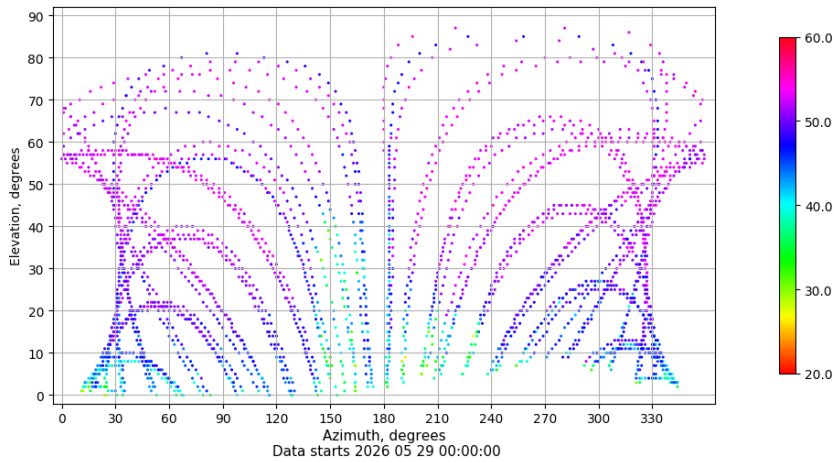
Azimuth-elevation plot for station EIVI. Signal to Noise S1C Data file EIVI00ESP_R_2026149.xtr
