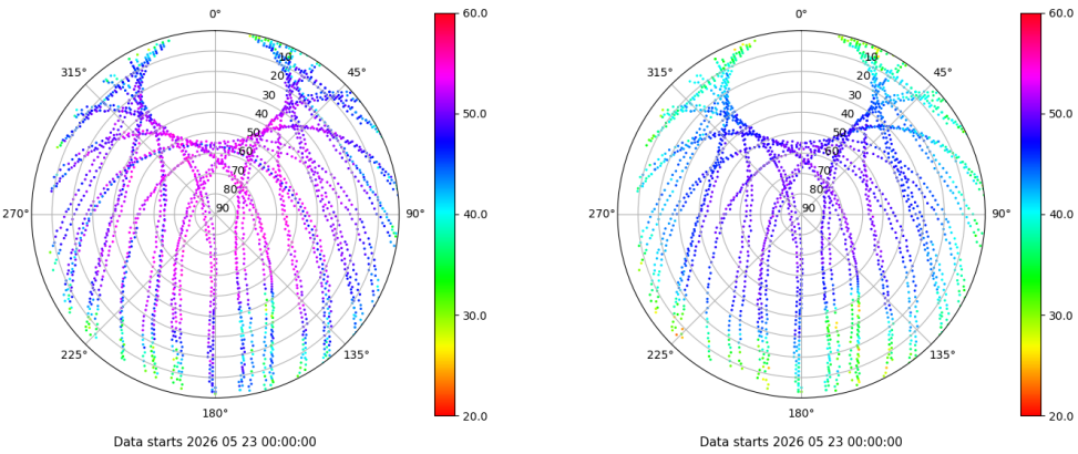
Skyplot for station EIVI. Signal to Noise S1C Data file EIVI00ESP_R_2026143.xtr Skyplot for station EIVI. Signal to Noise S2P Data file EIVI00ESP_R_2026143.xtr
