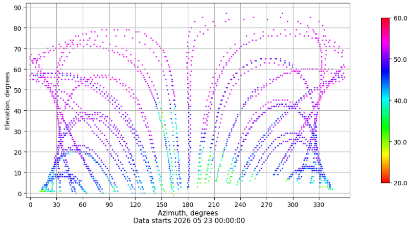
Azimuth-elevation plot for station EIVI. Signal to Noise S1C Data file EIVI00ESP_R_2026143.xtr
