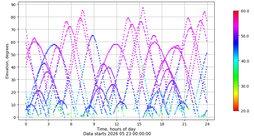
Time-elevation plot for station EIVI. Signal to Noise S1C Data file EIVI00ESP_R_2026143.xtr
