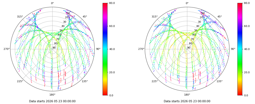
Skyplot for station EIVI. Parameter M1C Data file EIVI00ESP_R_2026143.xtr Skyplot for station EIVI. Parameter M2P Data file EIVI00ESP_R_2026143.xtr
