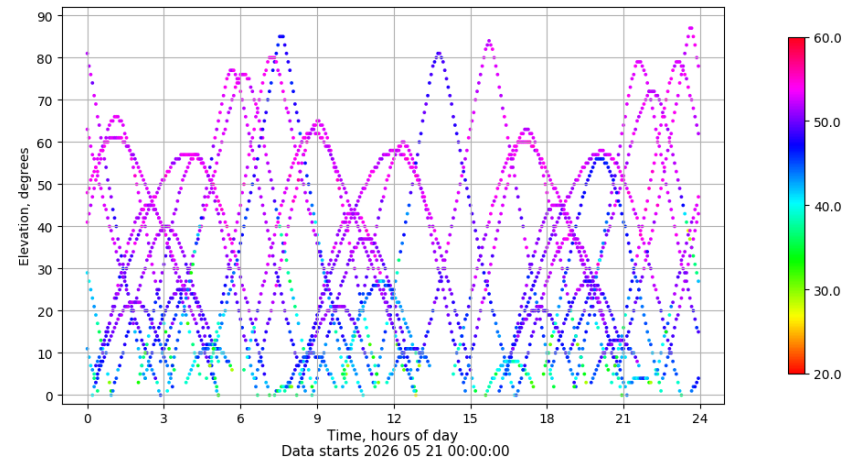
Time-elevation plot for station EIVI. Signal to Noise S1C Data file EIVI00ESP_R_2026141.xtr
