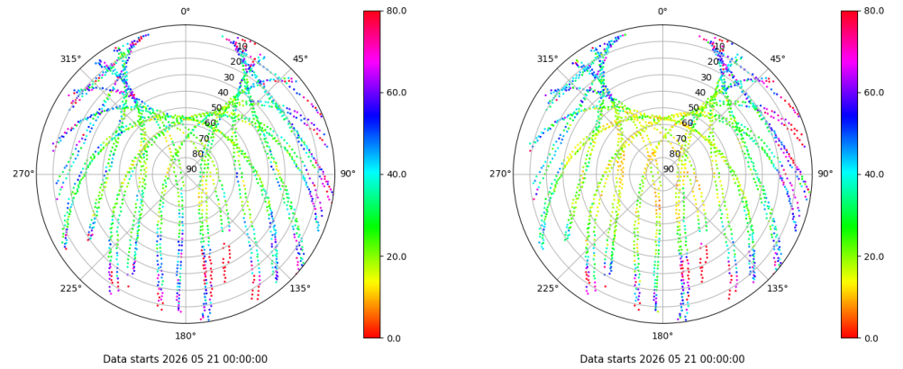
Skyplot for station EIVI. Parameter M1C Data file EIVI00ESP_R_2026141.xtr Skyplot for station EIVI. Parameter M2P Data file EIVI00ESP_R_2026141.xtr
