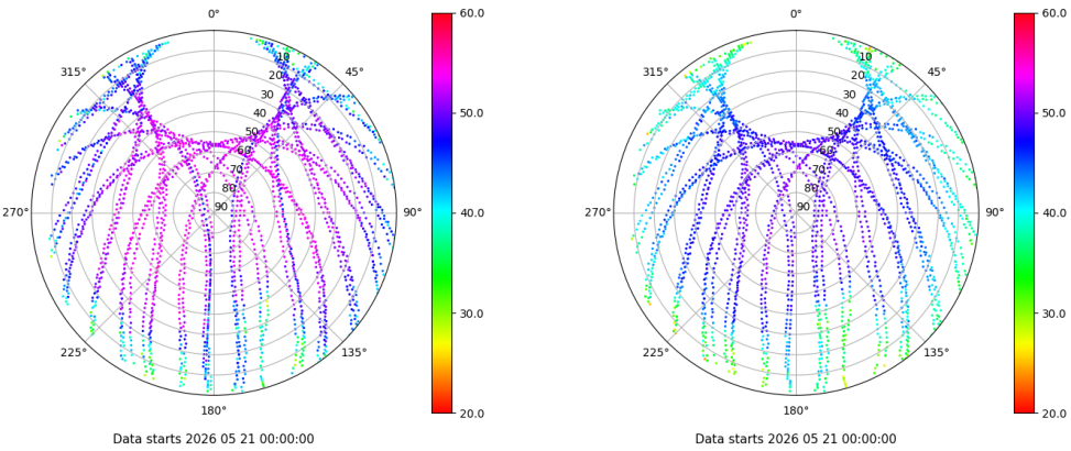
Skyplot for station EIVI. Signal to Noise S1C Data file EIVI00ESP_R_2026141.xtr Skyplot for station EIVI. Signal to Noise S2P Data file EIVI00ESP_R_2026141.xtr
