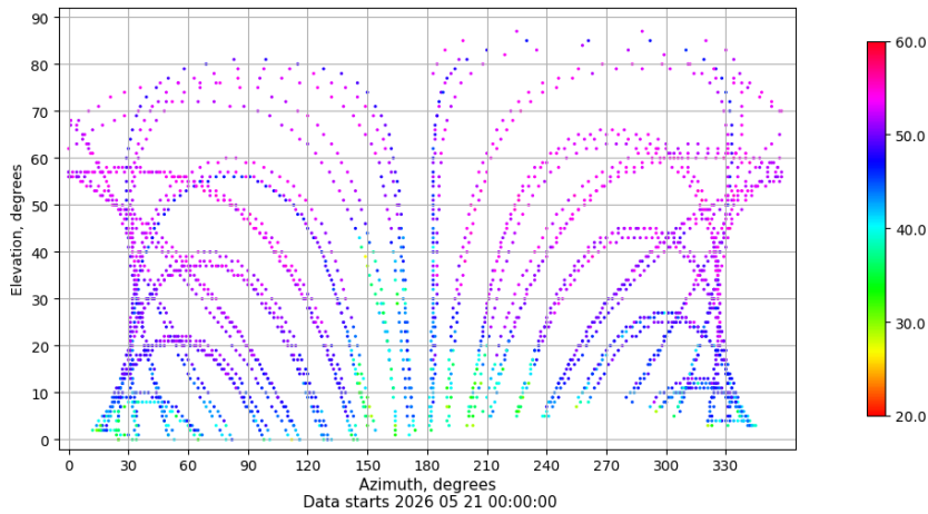
Azimuth-elevation plot for station EIVI. Signal to Noise S1C Data file EIVI00ESP_R_2026141.xtr
