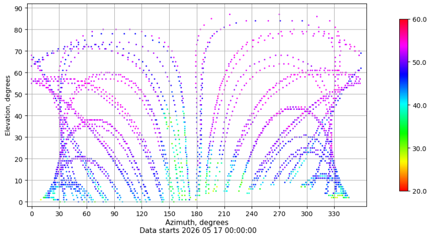
Azimuth-elevation plot for station EIVI. Signal to Noise S1C Data file EIVI00ESP_R_2026137.xtr
