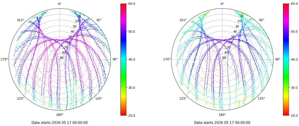
Skyplot for station EIVI. Signal to Noise S1C Data file EIVI00ESP_R_2026137.xtr Skyplot for station EIVI. Signal to Noise S2P Data file EIVI00ESP_R_2026137.xtr
