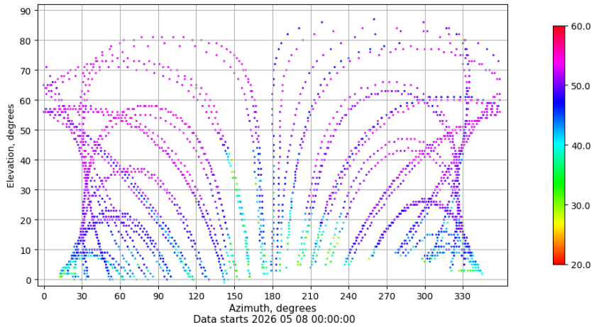
Azimuth-elevation plot for station EIVI. Signal to Noise S1C Data file EIVI00ESP_R_2026128.xtr
