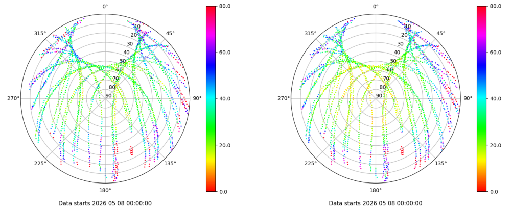
Skyplot for station EIVI. Parameter M1C Data file EIVI00ESP_R_2026128.xtr Skyplot for station EIVI. Parameter M2P Data file EIVI00ESP_R_2026128.xtr
