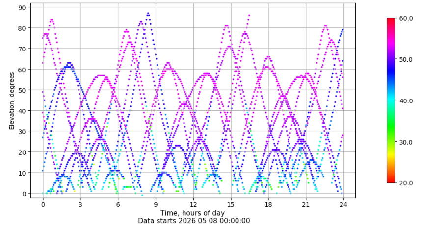
Time-elevation plot for station EIVI. Signal to Noise S1C Data file EIVI00ESP_R_2026128.xtr
