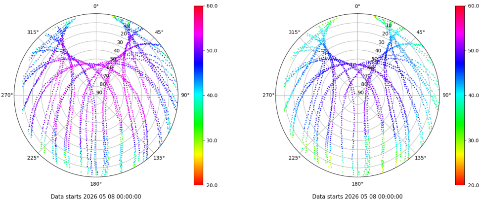
Skyplot for station EIVI. Signal to Noise S1C Data file EIVI00ESP_R_2026128.xtr Skyplot for station EIVI. Signal to Noise S2P Data file EIVI00ESP_R_2026128.xtr
