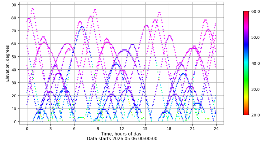
Time-elevation plot for station EIVI. Signal to Noise S1C Data file EIVI00ESP_R_2026126.xtr
