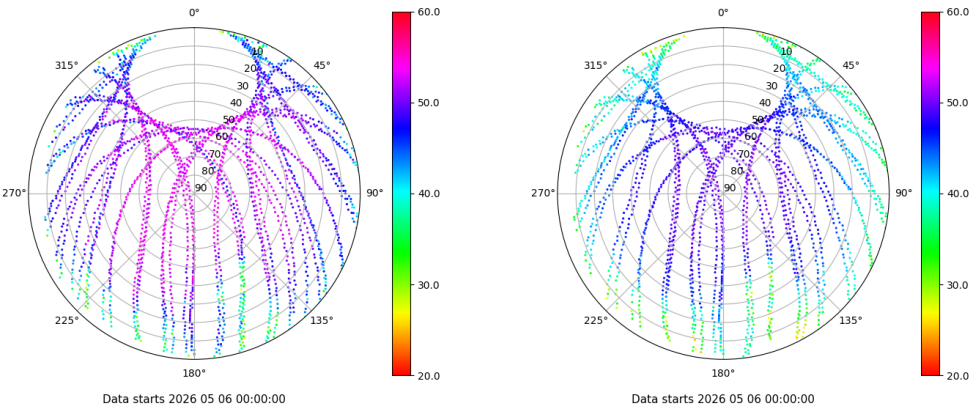
Skyplot for station EIVI. Signal to Noise S1C Data file EIVI00ESP_R_2026126.xtr Skyplot for station EIVI. Signal to Noise S2P Data file EIVI00ESP_R_2026126.xtr
