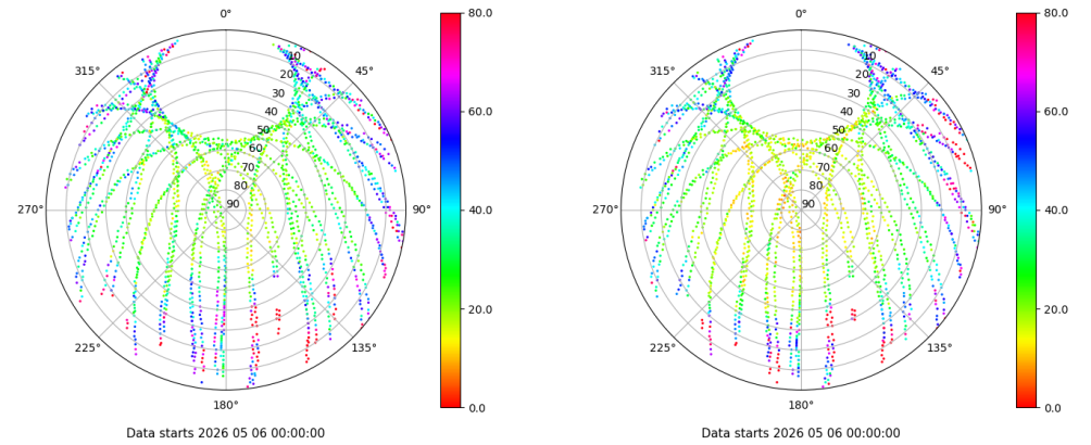
Skyplot for station EIVI. Parameter M1C Data file EIVI00ESP_R_2026126.xtr Skyplot for station EIVI. Parameter M2P Data file EIVI00ESP_R_2026126.xtr
