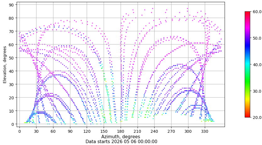
Azimuth-elevation plot for station EIVI. Signal to Noise S1C Data file EIVI00ESP_R_2026126.xtr
