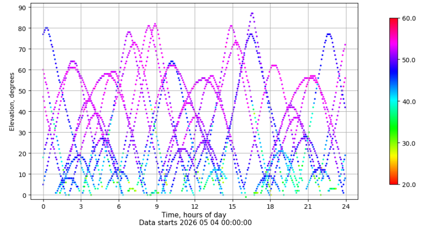
Time-elevation plot for station EIVI. Signal to Noise S1C Data file EIVI00ESP_R_2026124.xtr
