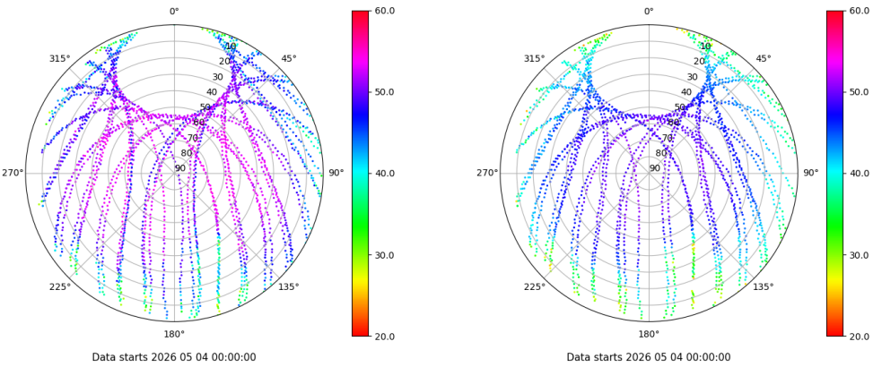
Skyplot for station EIVI. Signal to Noise S1C Data file EIVI00ESP_R_2026124.xtr Skyplot for station EIVI. Signal to Noise S2P Data file EIVI00ESP_R_2026124.xtr
