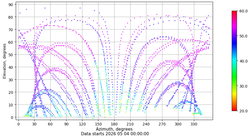
Azimuth-elevation plot for station EIVI. Signal to Noise S1C Data file EIVI00ESP_R_2026124.xtr
