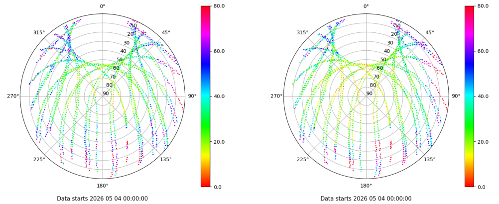
Skyplot for station EIVI. Parameter M1C Data file EIVI00ESP_R_2026124.xtr Skyplot for station EIVI. Parameter M2P Data file EIVI00ESP_R_2026124.xtr
