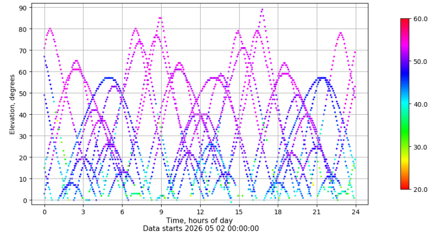
Time-elevation plot for station EIVI. Signal to Noise S1C Data file EIVI00ESP_R_2026122.xtr
