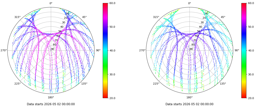
Skyplot for station EIVI. Signal to Noise S1C Data file EIVI00ESP_R_2026122.xtr Skyplot for station EIVI. Signal to Noise S2P Data file EIVI00ESP_R_2026122.xtr
