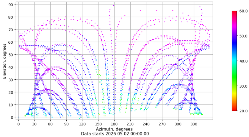
Azimuth-elevation plot for station EIVI. Signal to Noise S1C Data file EIVI00ESP_R_2026122.xtr
