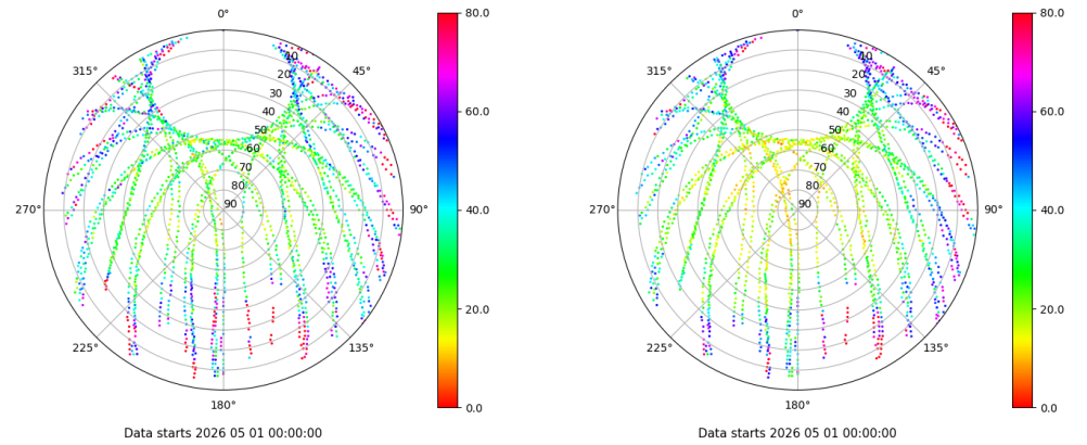
Skyplot for station EIVI. Parameter M1C Data file EIVI00ESP_R_2026121.xtr Skyplot for station EIVI. Parameter M2P Data file EIVI00ESP_R_2026121.xtr
