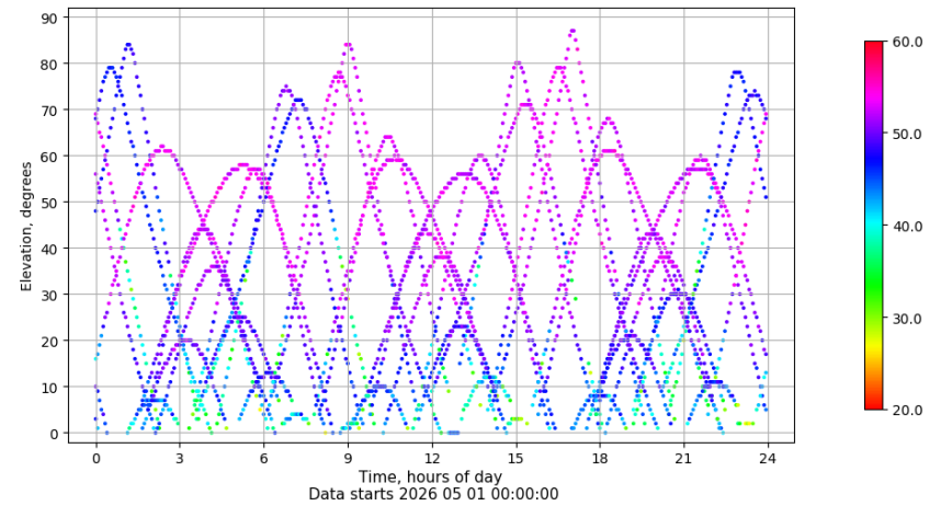
Time-elevation plot for station EIVI. Signal to Noise S1C Data file EIVI00ESP_R_2026121.xtr
