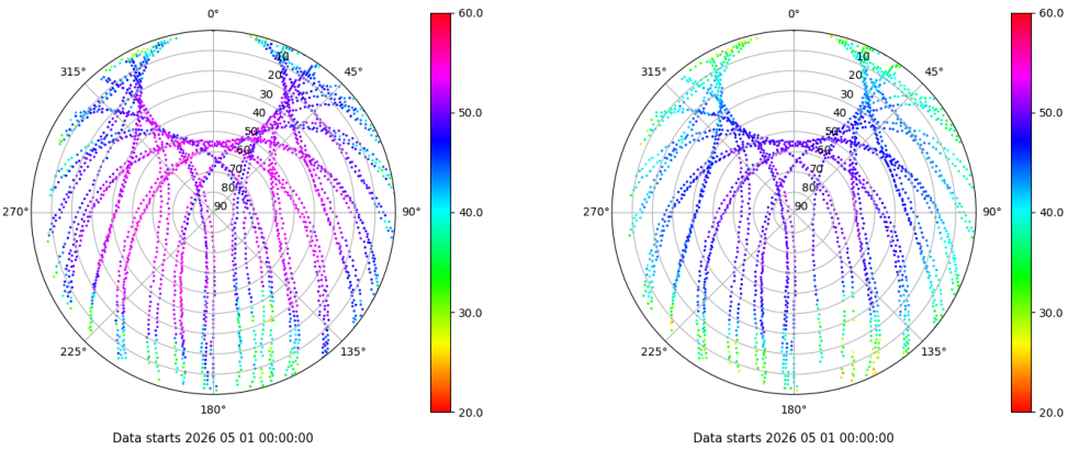
Skyplot for station EIVI. Signal to Noise S1C Data file EIVI00ESP_R_2026121.xtr Skyplot for station EIVI. Signal to Noise S2P Data file EIVI00ESP_R_2026121.xtr
