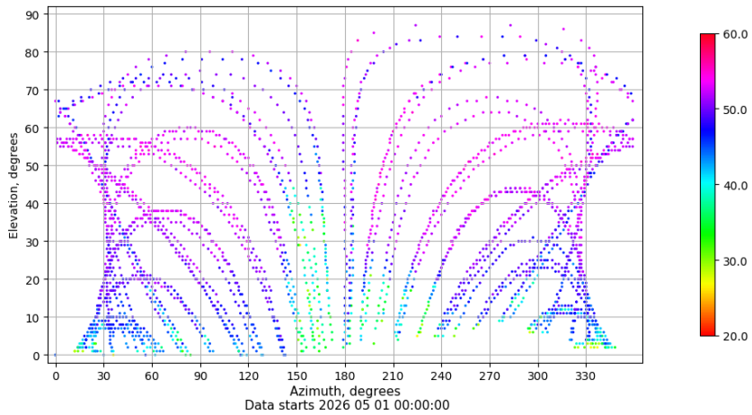
Azimuth-elevation plot for station EIVI. Signal to Noise S1C Data file EIVI00ESP_R_2026121.xtr
