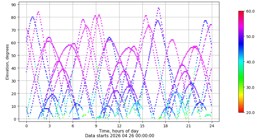
Time-elevation plot for station EIVI. Signal to Noise S1C Data file EIVI00ESP_R_2026116.xtr
