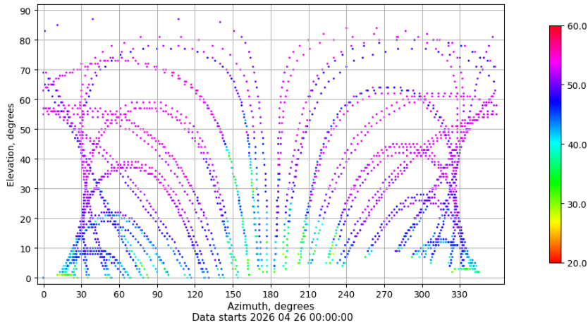
Azimuth-elevation plot for station EIVI. Signal to Noise S1C Data file EIVI00ESP_R_2026116.xtr
