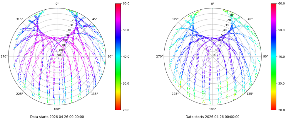
Skyplot for station EIVI. Signal to Noise S1C Data file EIVI00ESP_R_2026116.xtr Skyplot for station EIVI. Signal to Noise S2P Data file EIVI00ESP_R_2026116.xtr
