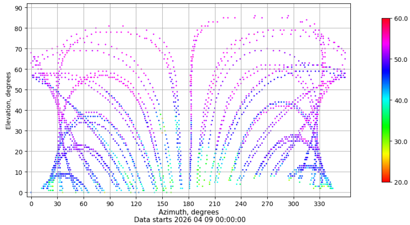
Azimuth-elevation plot for station EIVI. Signal to Noise S1C Data file EIVI00ESP_R_2026099.xtr
