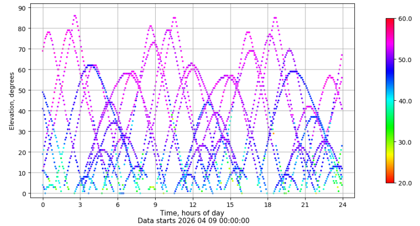
Time-elevation plot for station EIVI. Signal to Noise S1C Data file EIVI00ESP_R_2026099.xtr
