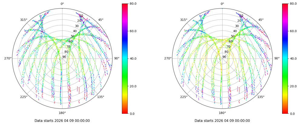
Skyplot for station EIVI. Parameter M1C Data file EIVI00ESP_R_2026099.xtr Skyplot for station EIVI. Parameter M2P Data file EIVI00ESP_R_2026099.xtr
