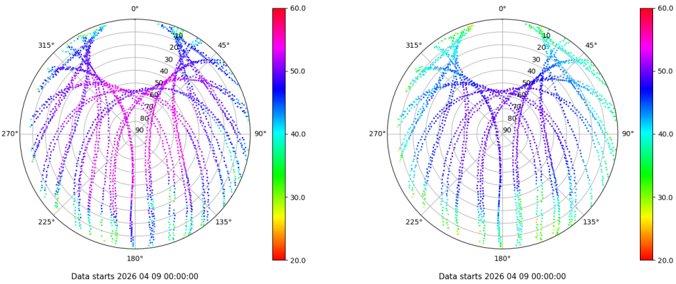
Skyplot for station EIVI. Signal to Noise S1C Data file EIVI00ESP_R_2026099.xtr Skyplot for station EIVI. Signal to Noise S2P Data file EIVI00ESP_R_2026099.xtr
