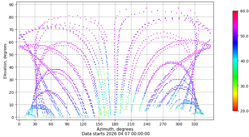
Azimuth-elevation plot for station EIVI. Signal to Noise S1C Data file EIVI00ESP_R_2026097.xtr
