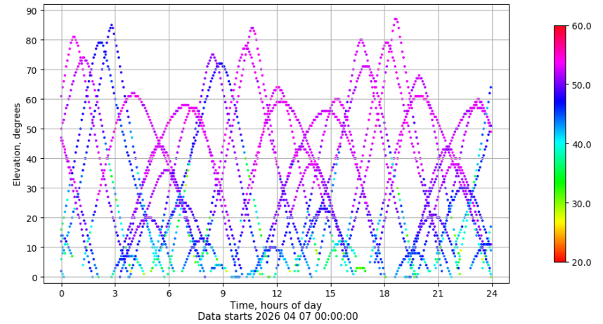
Time-elevation plot for station EIVI. Signal to Noise S1C Data file EIVI00ESP_R_2026097.xtr
