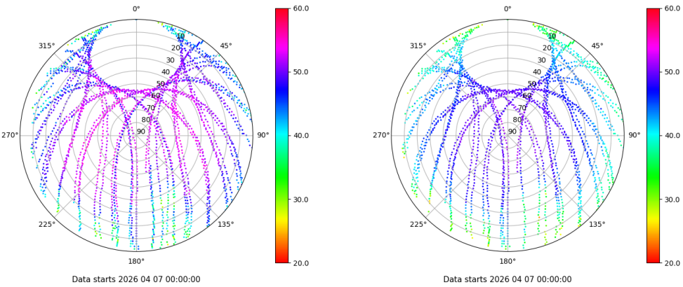
Skyplot for station EIVI. Signal to Noise S1C Data file EIVI00ESP_R_2026097.xtr Skyplot for station EIVI. Signal to Noise S2P Data file EIVI00ESP_R_2026097.xtr
