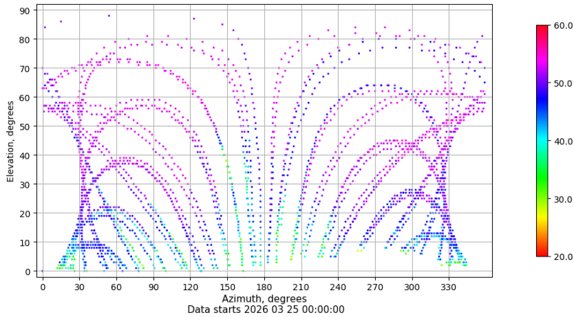
Azimuth-elevation plot for station EIVI. Signal to Noise S1C Data file EIVI00ESP_R_2026084.xtr
