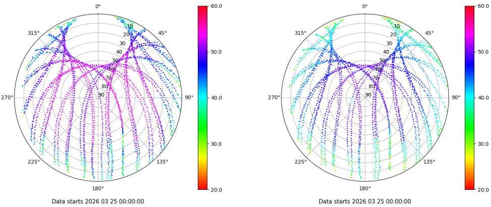
Skyplot for station EIVI. Signal to Noise S1C Data file EIVI00ESP_R_2026084.xtr Skyplot for station EIVI. Signal to Noise S2P Data file EIVI00ESP_R_2026084.xtr
