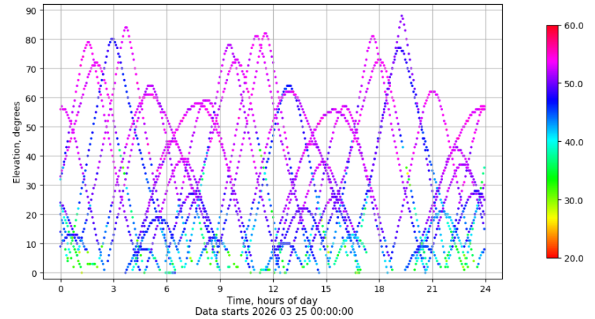
Time-elevation plot for station EIVI. Signal to Noise S1C Data file EIVI00ESP_R_2026084.xtr
