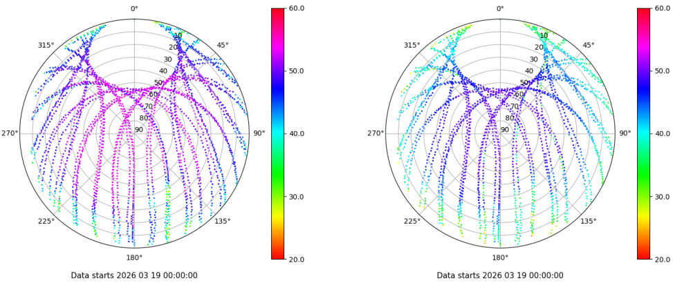
Skyplot for station EIVI. Signal to Noise S1C Data file EIVI00ESP_R_2026078.xtr Skyplot for station EIVI. Signal to Noise S2P Data file EIVI00ESP_R_2026078.xtr
