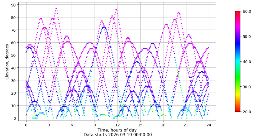
Time-elevation plot for station EIVI. Signal to Noise S1C Data file EIVI00ESP_R_2026078.xtr
