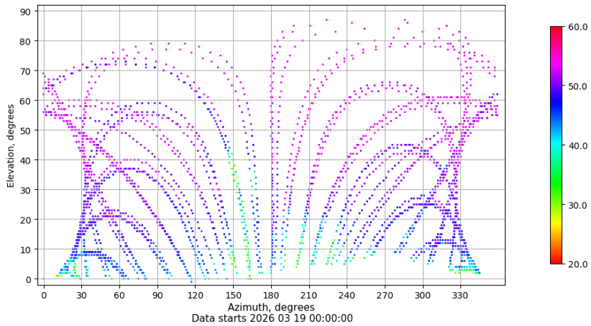
Azimuth-elevation plot for station EIVI. Signal to Noise S1C Data file EIVI00ESP_R_2026078.xtr
