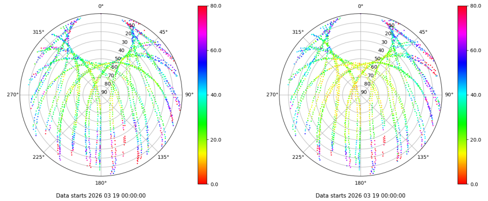
Skyplot for station EIVI. Parameter M1C Data file EIVI00ESP_R_2026078.xtr Skyplot for station EIVI. Parameter M2P Data file EIVI00ESP_R_2026078.xtr
