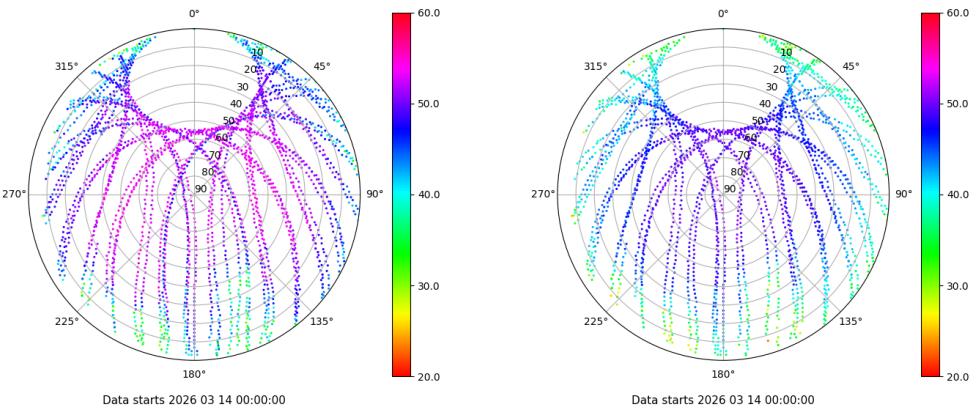
Skyplot for station EIVI. Signal to Noise S1C Data file EIVI00ESP_R_2026073.xtr Skyplot for station EIVI. Signal to Noise S2P Data file EIVI00ESP_R_2026073.xtr
