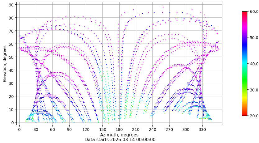
Azimuth-elevation plot for station EIVI. Signal to Noise S1C Data file EIVI00ESP_R_2026073.xtr
