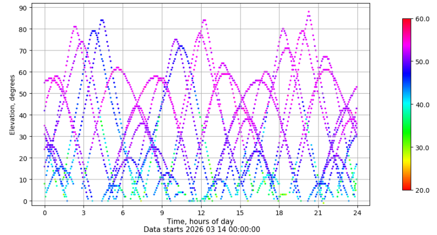
Time-elevation plot for station EIVI. Signal to Noise S1C Data file EIVI00ESP_R_2026073.xtr
