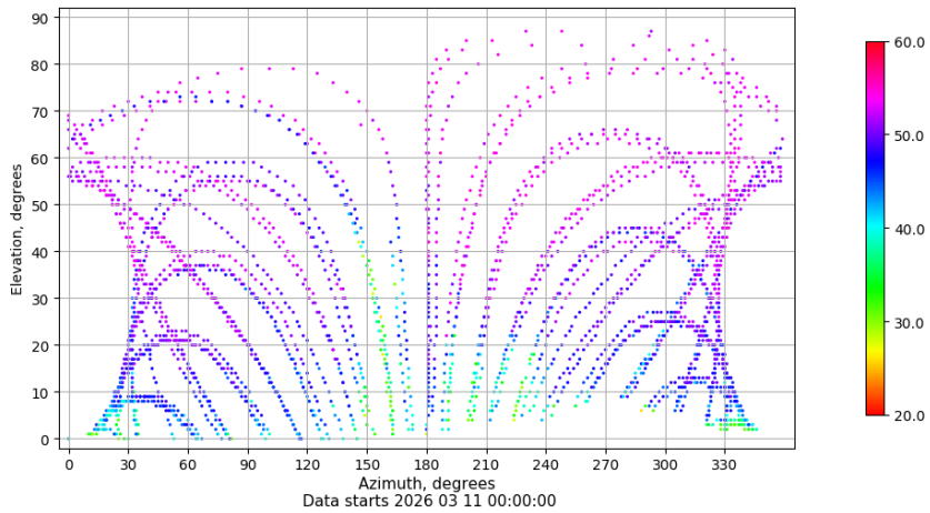
Azimuth-elevation plot for station EIVI. Signal to Noise S1C Data file EIVI00ESP_R_2026070.xtr
