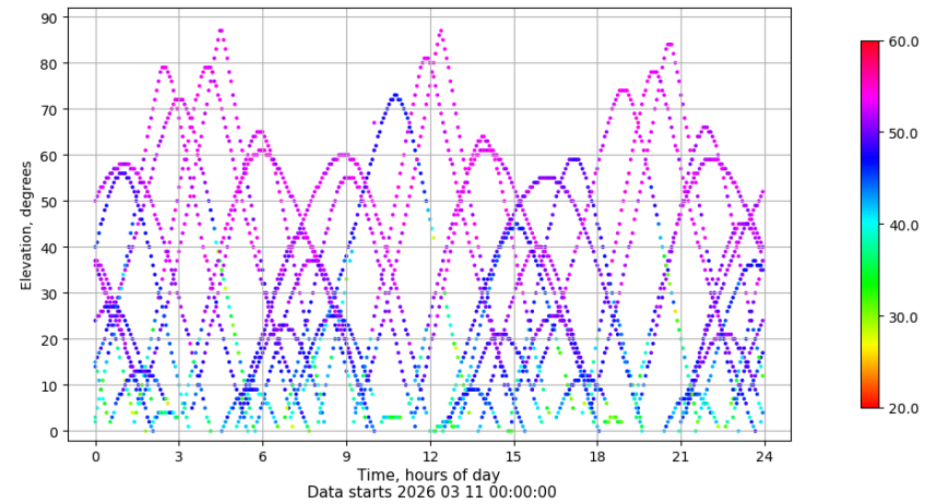
Time-elevation plot for station EIVI. Signal to Noise S1C Data file EIVI00ESP_R_2026070.xtr
