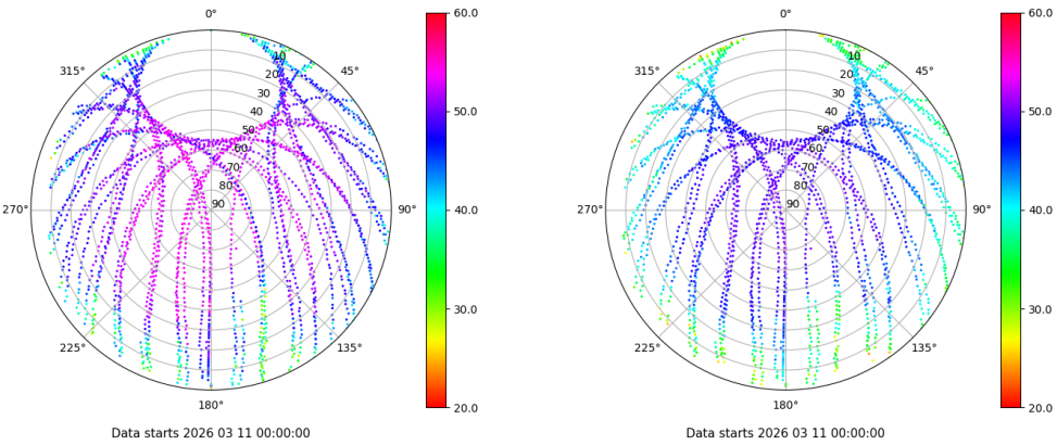
Skyplot for station EIVI. Signal to Noise S1C Data file EIVI00ESP_R_2026070.xtr Skyplot for station EIVI. Signal to Noise S2P Data file EIVI00ESP_R_2026070.xtr
