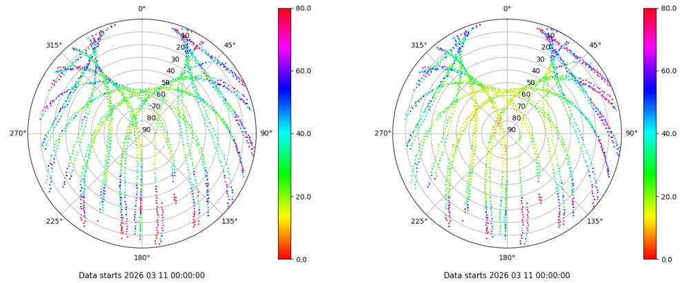
Skyplot for station EIVI. Parameter M1C Data file EIVI00ESP_R_2026070.xtr Skyplot for station EIVI. Parameter M2P Data file EIVI00ESP_R_2026070.xtr
