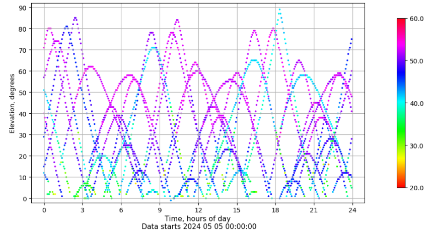
Time-elevation plot for station EIVI. Signal to Noise S1C Data file EIVI00ESP_R_2024126.xtr
