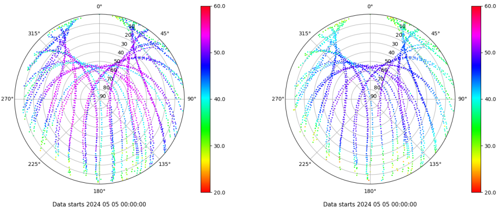
Skyplot for station EIVI. Signal to Noise S1C Data file EIVI00ESP_R_2024126.xtr Skyplot for station EIVI. Signal to Noise S2P Data file EIVI00ESP_R_2024126.xtr
