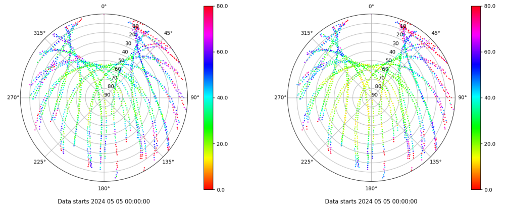
Skyplot for station EIVI. Parameter M1C Data file EIVI00ESP_R_2024126.xtr Skyplot for station EIVI. Parameter M2P Data file EIVI00ESP_R_2024126.xtr
