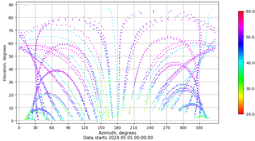
Azimuth-elevation plot for station EIVI. Signal to Noise S1C Data file EIVI00ESP_R_2024126.xtr
