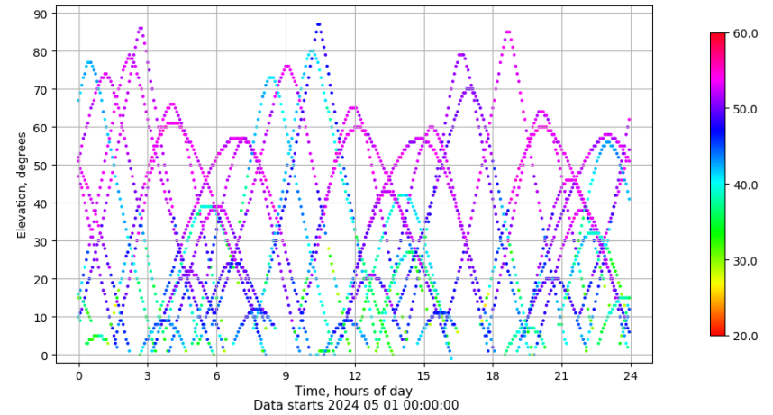
Time-elevation plot for station EIVI. Signal to Noise S1C Data file EIVI00ESP_R_2024122.xtr
