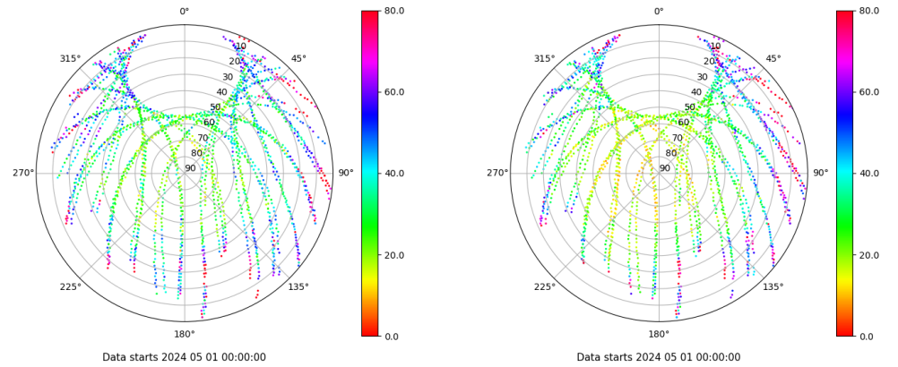
Skyplot for station EIVI. Parameter M1C Data file EIVI00ESP_R_2024122.xtr Skyplot for station EIVI. Parameter M2P Data file EIVI00ESP_R_2024122.xtr
