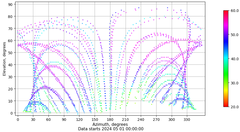
Azimuth-elevation plot for station EIVI. Signal to Noise S1C Data file EIVI00ESP_R_2024122.xtr
