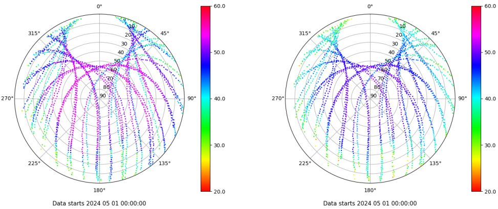
Skyplot for station EIVI. Signal to Noise S1C Data file EIVI00ESP_R_2024122.xtr Skyplot for station EIVI. Signal to Noise S2P Data file EIVI00ESP_R_2024122.xtr
