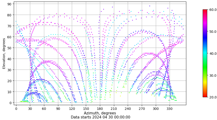
Azimuth-elevation plot for station EIVI. Signal to Noise S1C Data file EIVI00ESP_R_2024121.xtr
