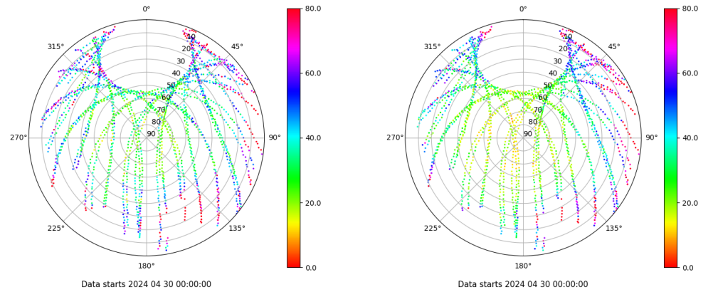
Skyplot for station EIVI. Parameter M1C Data file EIVI00ESP_R_2024121.xtr Skyplot for station EIVI. Parameter M2P Data file EIVI00ESP_R_2024121.xtr
