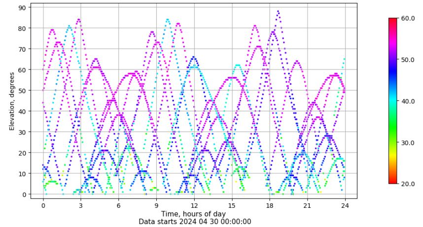
Time-elevation plot for station EIVI. Signal to Noise S1C Data file EIVI00ESP_R_2024121.xtr
