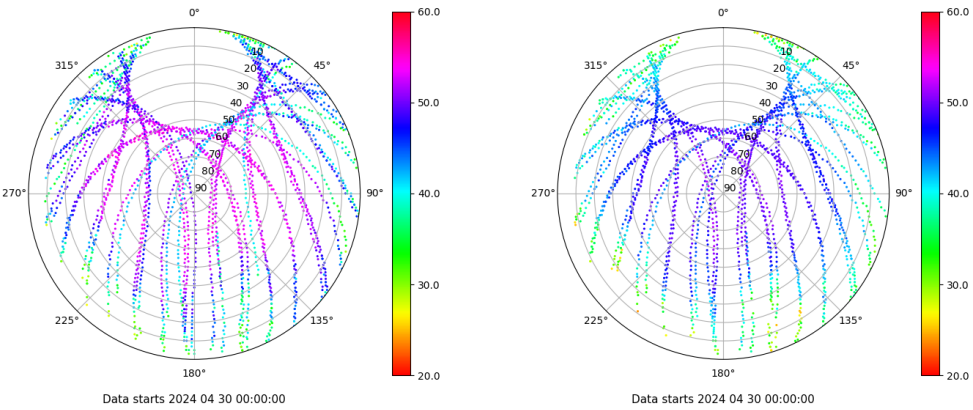
Skyplot for station EIVI. Signal to Noise S1C Data file EIVI00ESP_R_2024121.xtr Skyplot for station EIVI. Signal to Noise S2P Data file EIVI00ESP_R_2024121.xtr
