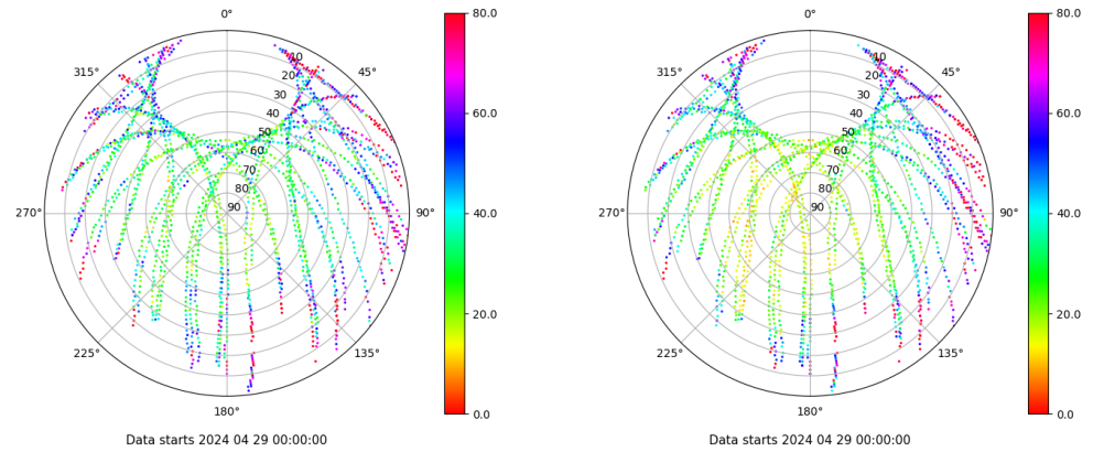
Skyplot for station EIVI. Parameter M1C Data file EIVI00ESP_R_2024120.xtr Skyplot for station EIVI. Parameter M2P Data file EIVI00ESP_R_2024120.xtr
