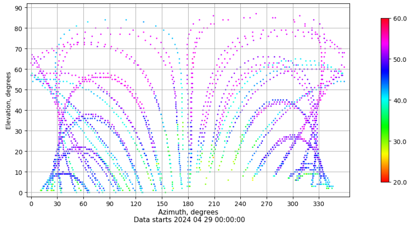
Azimuth-elevation plot for station EIVI. Signal to Noise S1C Data file EIVI00ESP_R_2024120.xtr
