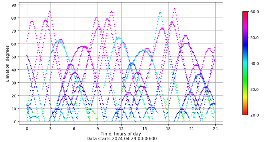
Time-elevation plot for station EIVI. Signal to Noise S1C Data file EIVI00ESP_R_2024120.xtr
