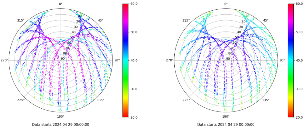
Skyplot for station EIVI. Signal to Noise S1C Data file EIVI00ESP_R_2024120.xtr Skyplot for station EIVI. Signal to Noise S2P Data file EIVI00ESP_R_2024120.xtr
