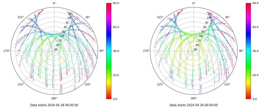
Skyplot for station EIVI. Parameter M1C Data file EIVI00ESP_R_2024119.xtr Skyplot for station EIVI. Parameter M2P Data file EIVI00ESP_R_2024119.xtr
