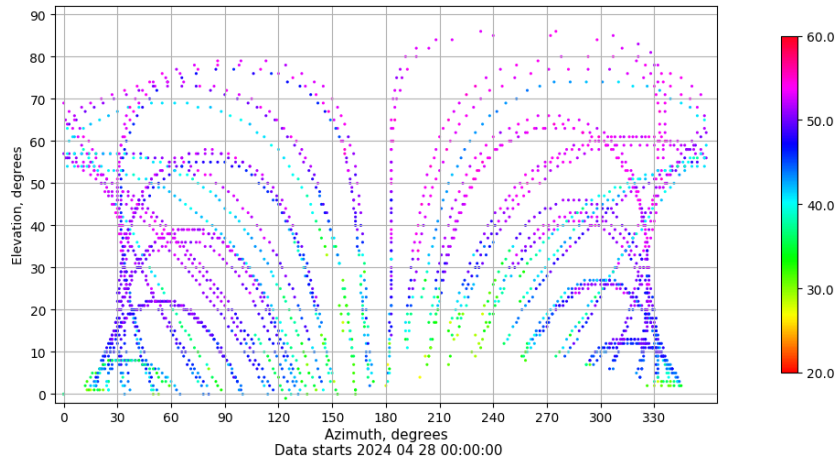
Azimuth-elevation plot for station EIVI. Signal to Noise S1C Data file EIVI00ESP_R_2024119.xtr
