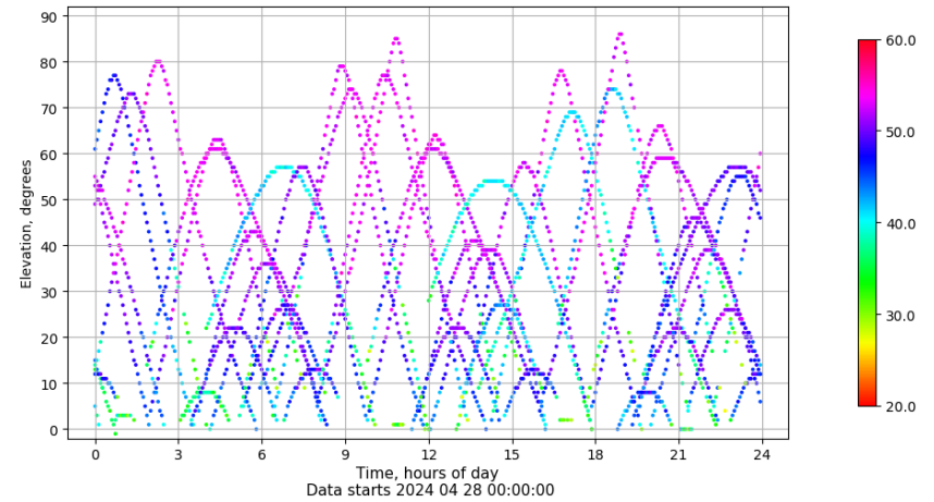
Time-elevation plot for station EIVI. Signal to Noise S1C Data file EIVI00ESP_R_2024119.xtr
