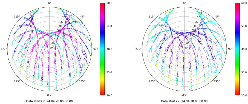
Skyplot for station EIVI. Signal to Noise S1C Data file EIVI00ESP_R_2024119.xtr Skyplot for station EIVI. Signal to Noise S2P Data file EIVI00ESP_R_2024119.xtr
