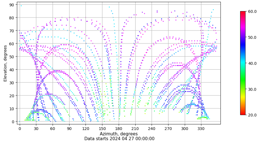
Azimuth-elevation plot for station EIVI. Signal to Noise S1C Data file EIVI00ESP_R_2024118.xtr
