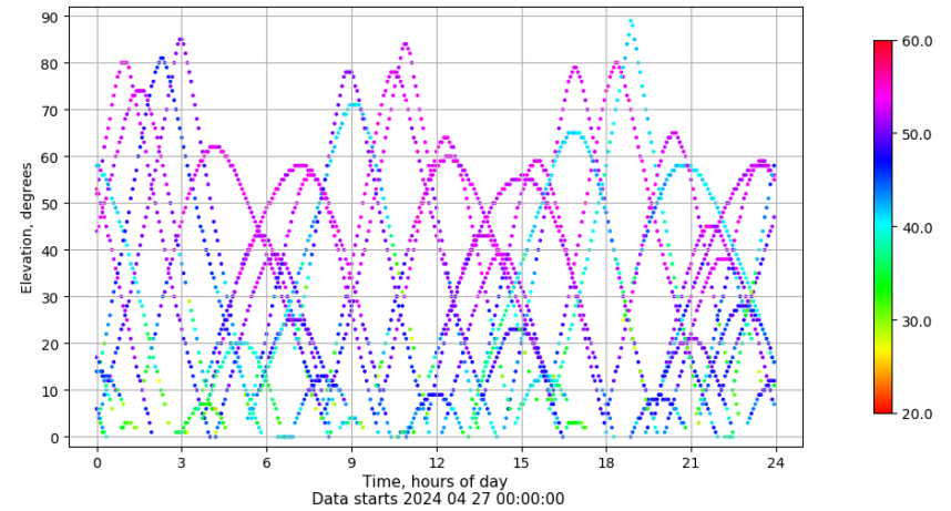
Time-elevation plot for station EIVI. Signal to Noise S1C Data file EIVI00ESP_R_2024118.xtr
