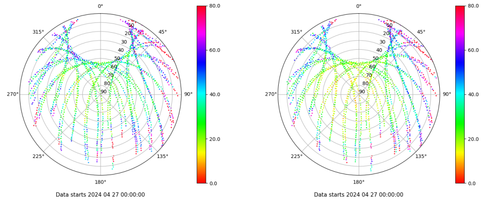
Skyplot for station EIVI. Parameter M1C Data file EIVI00ESP_R_2024118.xtr Skyplot for station EIVI. Parameter M2P Data file EIVI00ESP_R_2024118.xtr
