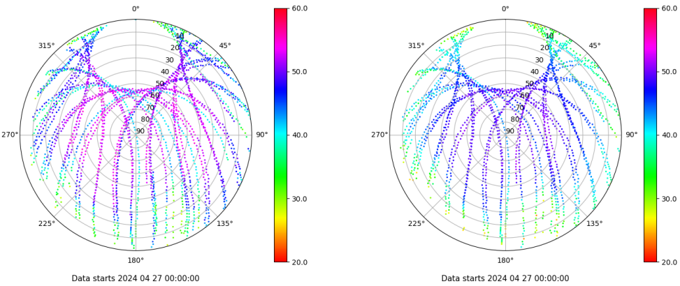
Skyplot for station EIVI. Signal to Noise S1C Data file EIVI00ESP_R_2024118.xtr Skyplot for station EIVI. Signal to Noise S2P Data file EIVI00ESP_R_2024118.xtr
