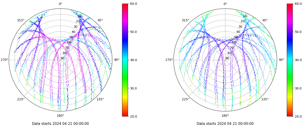
Skyplot for station EIVI. Signal to Noise S1C Data file EIVI00ESP_R_2024112.xtr Skyplot for station EIVI. Signal to Noise S2P Data file EIVI00ESP_R_2024112.xtr
