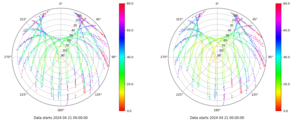
Skyplot for station EIVI. Parameter M1C Data file EIVI00ESP_R_2024112.xtr Skyplot for station EIVI. Parameter M2P Data file EIVI00ESP_R_2024112.xtr
