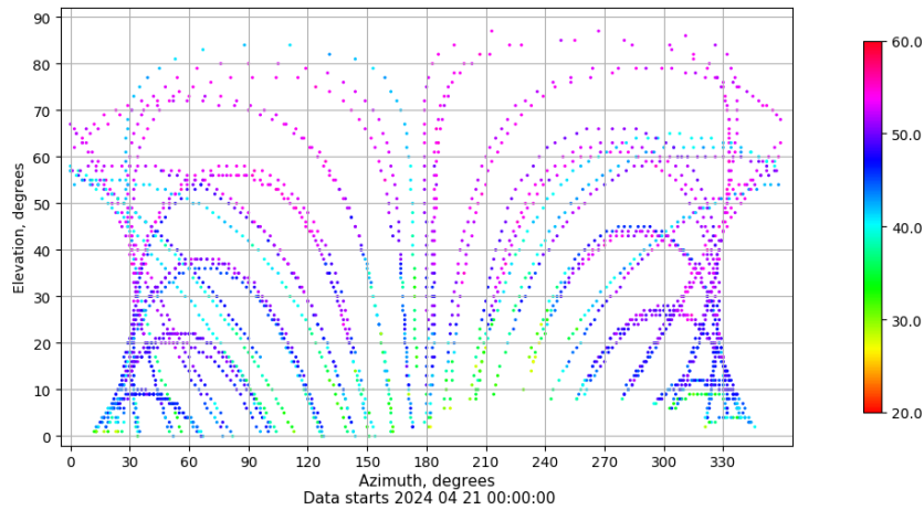
Azimuth-elevation plot for station EIVI. Signal to Noise S1C Data file EIVI00ESP_R_2024112.xtr
