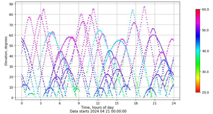
Time-elevation plot for station EIVI. Signal to Noise S1C Data file EIVI00ESP_R_2024112.xtr
