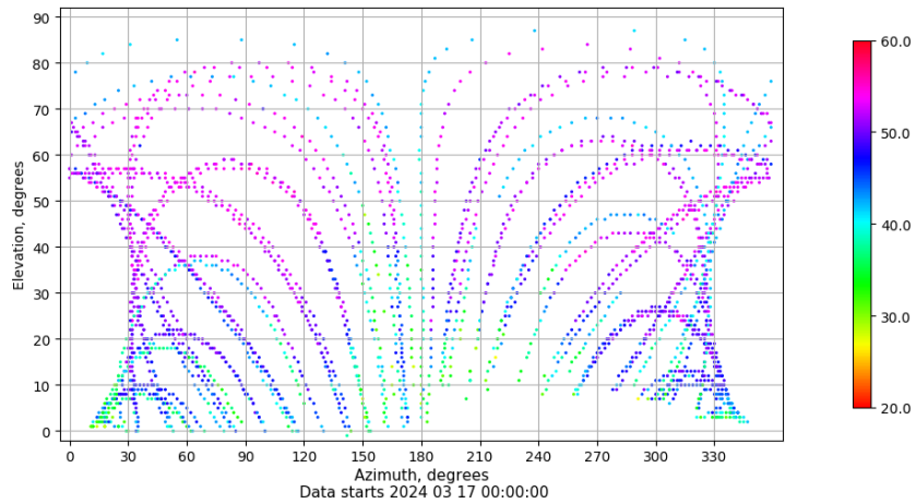
Azimuth-elevation plot for station EIVI. Signal to Noise S1C Data file EIVI00ESP_R_2024077.xtr
