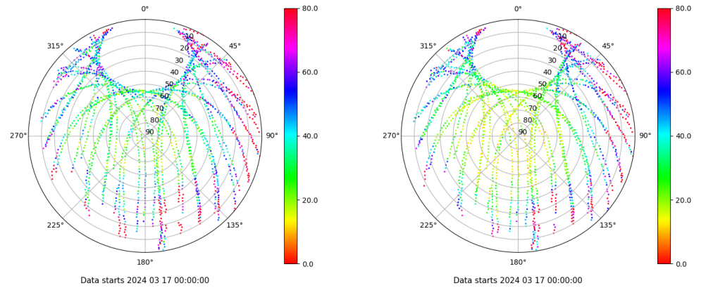
Skyplot for station EIVI. Parameter M1C Data file EIVI00ESP_R_2024077.xtr Skyplot for station EIVI. Parameter M2P Data file EIVI00ESP_R_2024077.xtr
