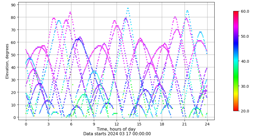
Time-elevation plot for station EIVI. Signal to Noise S1C Data file EIVI00ESP_R_2024077.xtr
