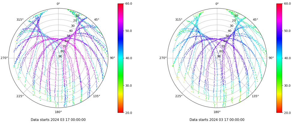
Skyplot for station EIVI. Signal to Noise S1C Data file EIVI00ESP_R_2024077.xtr Skyplot for station EIVI. Signal to Noise S2P Data file EIVI00ESP_R_2024077.xtr
