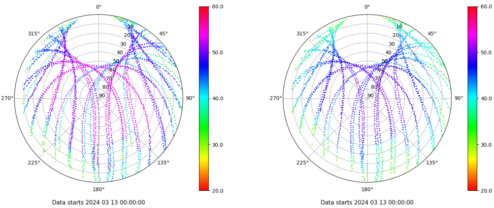
Skyplot for station EIVI. Signal to Noise S1C Data file EIVI00ESP_R_2024073.xtr Skyplot for station EIVI. Signal to Noise S2P Data file EIVI00ESP_R_2024073.xtr
