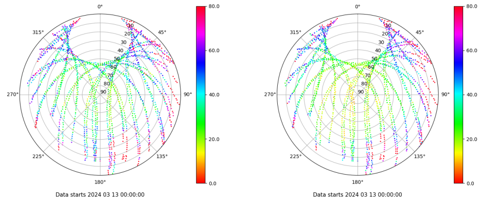
Skyplot for station EIVI. Parameter M1C Data file EIVI00ESP_R_2024073.xtr Skyplot for station EIVI. Parameter M2P Data file EIVI00ESP_R_2024073.xtr
