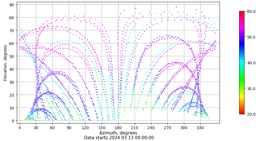
Azimuth-elevation plot for station EIVI. Signal to Noise S1C Data file EIVI00ESP_R_2024073.xtr
