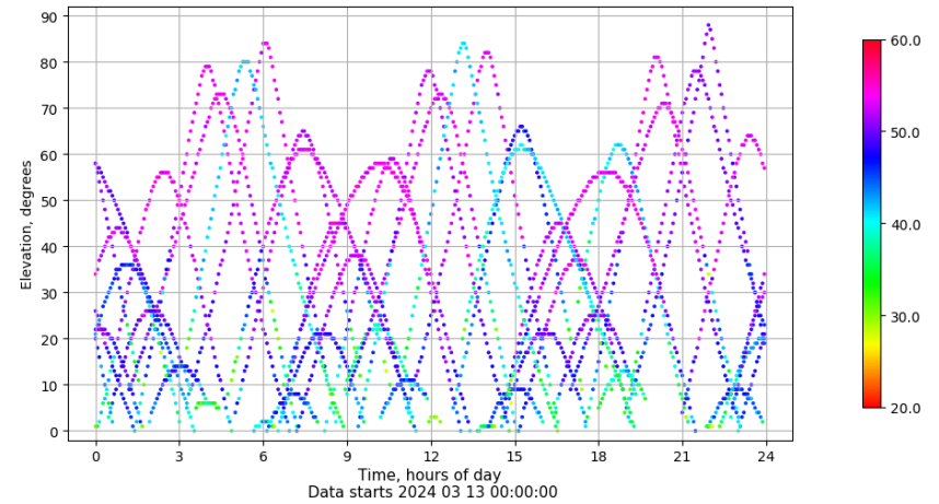
Time-elevation plot for station EIVI. Signal to Noise S1C Data file EIVI00ESP_R_2024073.xtr
