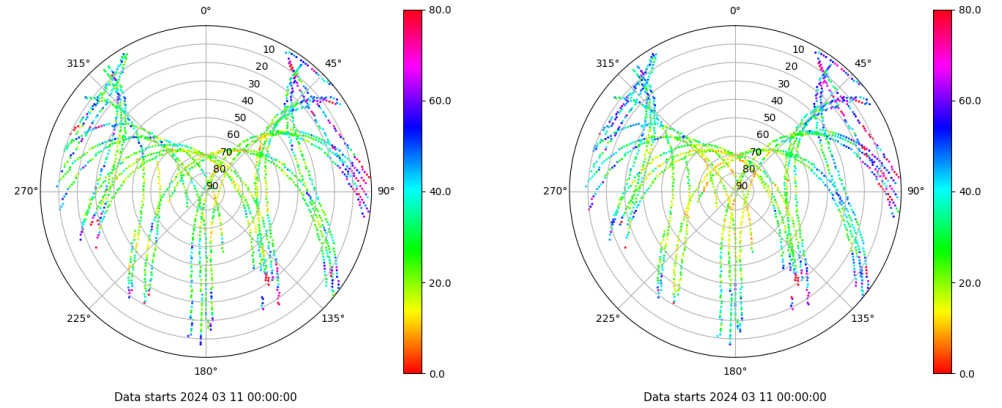
Skyplot for station EIVI. Parameter M1C Data file EIVI00ESP_R_2024071.xtr Skyplot for station EIVI. Parameter M5Q Data file EIVI00ESP_R_2024071.xtr
