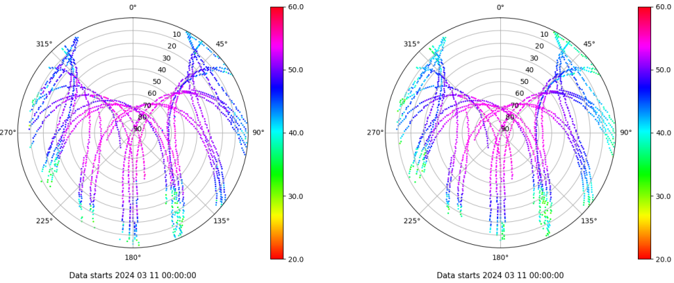
Skyplot for station EIVI. Signal to Noise S1C Data file EIVI00ESP_R_2024071.xtr Skyplot for station EIVI. Signal to Noise S5Q Data file EIVI00ESP_R_2024071.xtr
