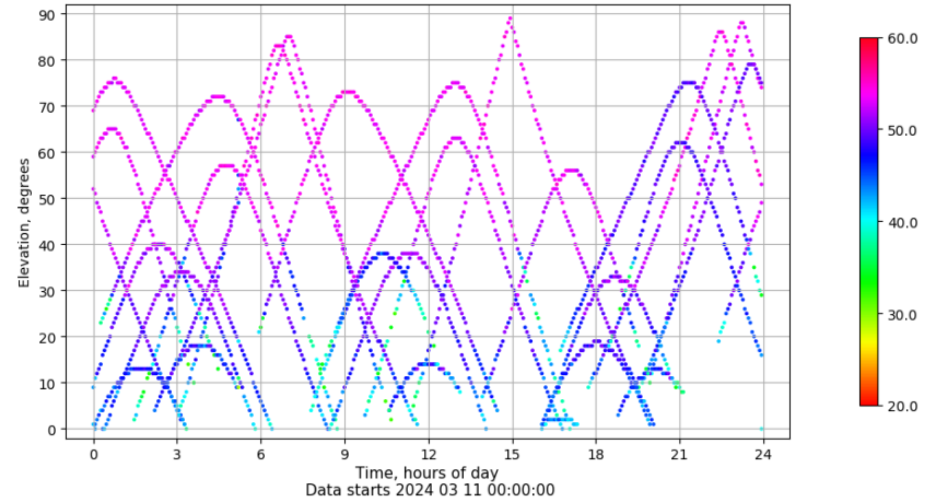
Time-elevation plot for station EIVI. Signal to Noise S1C Data file EIVI00ESP_R_2024071.xtr
