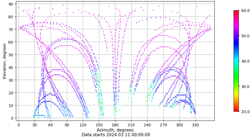
Azimuth-elevation plot for station EIVI. Signal to Noise S1C Data file EIVI00ESP_R_2024071.xtr
