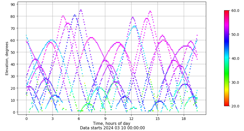
Time-elevation plot for station EIVI. Signal to Noise S1C Data file EIVI00ESP_R_2024070.xtr
