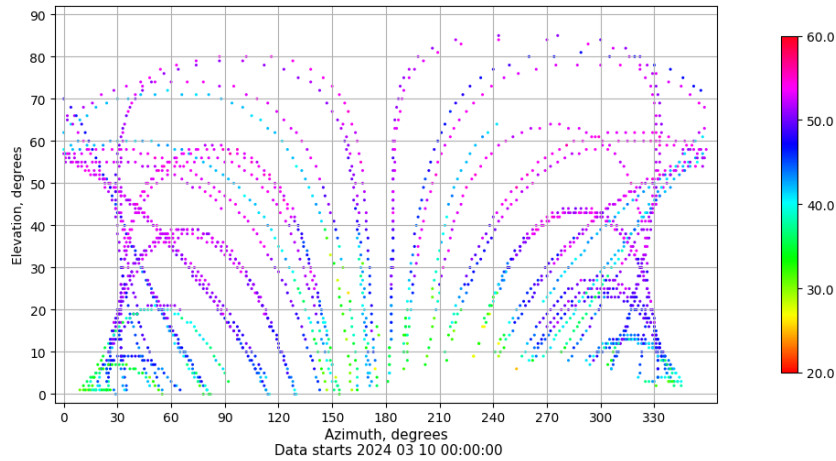
Azimuth-elevation plot for station EIVI. Signal to Noise S1C Data file EIVI00ESP_R_2024070.xtr
