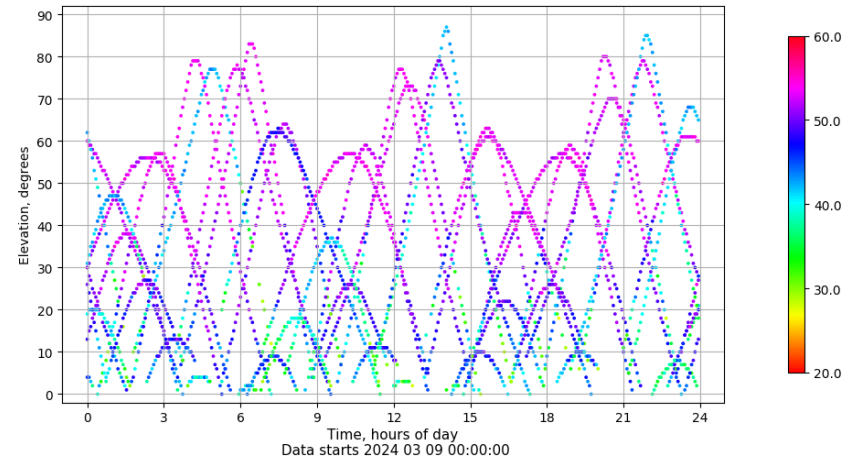
Time-elevation plot for station EIVI. Signal to Noise S1C Data file EIVI00ESP_R_2024069.xtr
