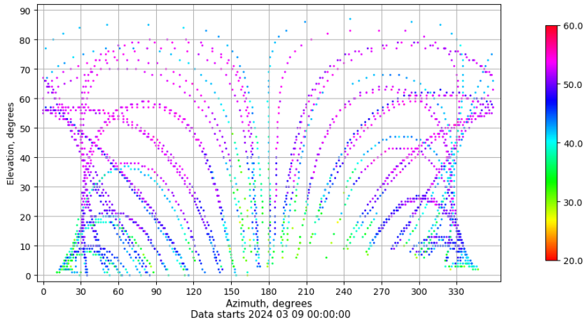
Azimuth-elevation plot for station EIVI. Signal to Noise S1C Data file EIVI00ESP_R_2024069.xtr
