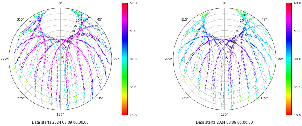
Skyplot for station EIVI. Signal to Noise S1C Data file EIVI00ESP_R_2024069.xtr Skyplot for station EIVI. Signal to Noise S2P Data file EIVI00ESP_R_2024069.xtr
