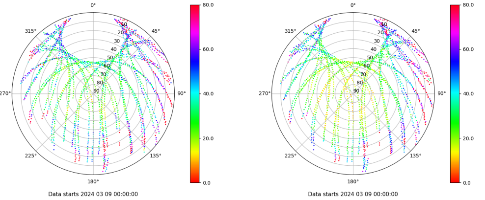
Skyplot for station EIVI. Parameter M1C Data file EIVI00ESP_R_2024069.xtr Skyplot for station EIVI. Parameter M2P Data file EIVI00ESP_R_2024069.xtr
