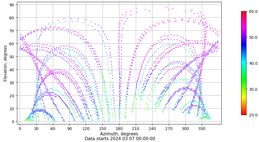
Azimuth-elevation plot for station EIVI. Signal to Noise S1C Data file EIVI00ESP_R_2024067.xtr
