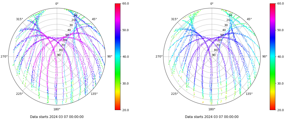
Skyplot for station EIVI. Signal to Noise S1C Data file EIVI00ESP_R_2024067.xtr Skyplot for station EIVI. Signal to Noise S2P Data file EIVI00ESP_R_2024067.xtr
