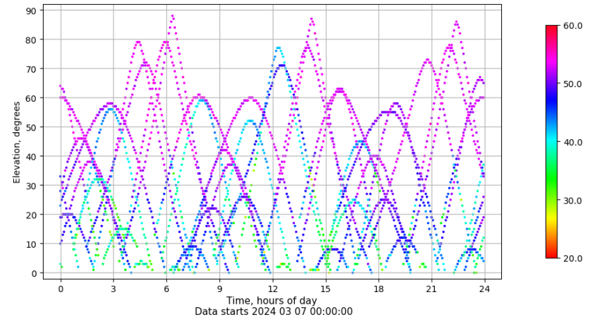
Time-elevation plot for station EIVI. Signal to Noise S1C Data file EIVI00ESP_R_2024067.xtr
