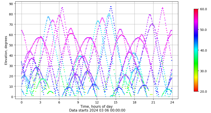
Time-elevation plot for station EIVI. Signal to Noise S1C Data file EIVI00ESP_R_2024066.xtr
