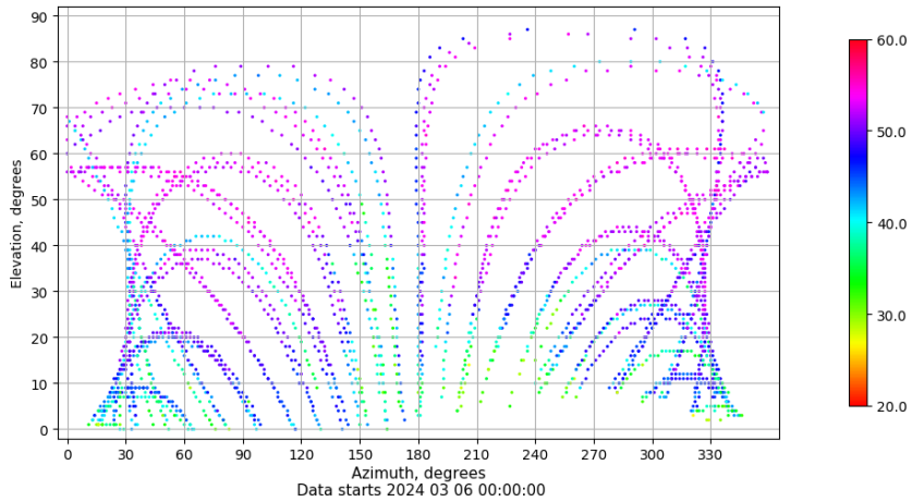
Azimuth-elevation plot for station EIVI. Signal to Noise S1C Data file EIVI00ESP_R_2024066.xtr
