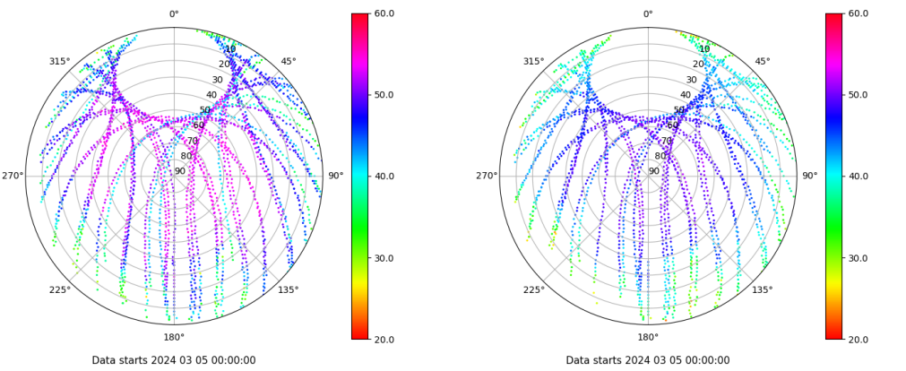
Skyplot for station EIVI. Signal to Noise S1C Data file EIVI00ESP_R_2024065.xtr Skyplot for station EIVI. Signal to Noise S2P Data file EIVI00ESP_R_2024065.xtr
