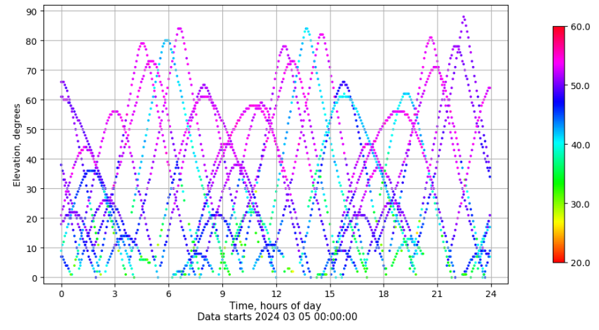
Time-elevation plot for station EIVI. Signal to Noise S1C Data file EIVI00ESP_R_2024065.xtr
