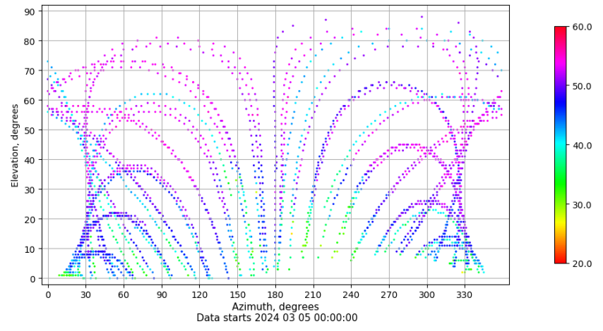
Azimuth-elevation plot for station EIVI. Signal to Noise S1C Data file EIVI00ESP_R_2024065.xtr
