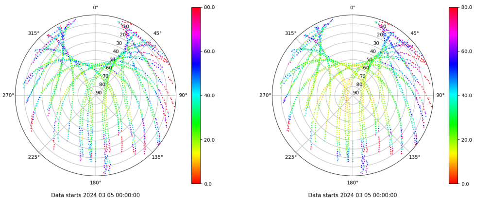
Skyplot for station EIVI. Parameter M1C Data file EIVI00ESP_R_2024065.xtr Skyplot for station EIVI. Parameter M2P Data file EIVI00ESP_R_2024065.xtr
