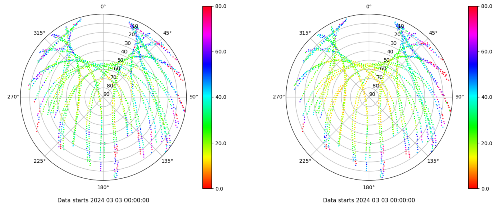
Skyplot for station EIVI. Parameter M1C Data file EIVI00ESP_R_2024063.xtr Skyplot for station EIVI. Parameter M2P Data file EIVI00ESP_R_2024063.xtr
