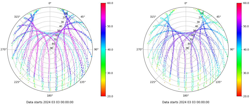
Skyplot for station EIVI. Signal to Noise S1C Data file EIVI00ESP_R_2024063.xtr Skyplot for station EIVI. Signal to Noise S2P Data file EIVI00ESP_R_2024063.xtr
