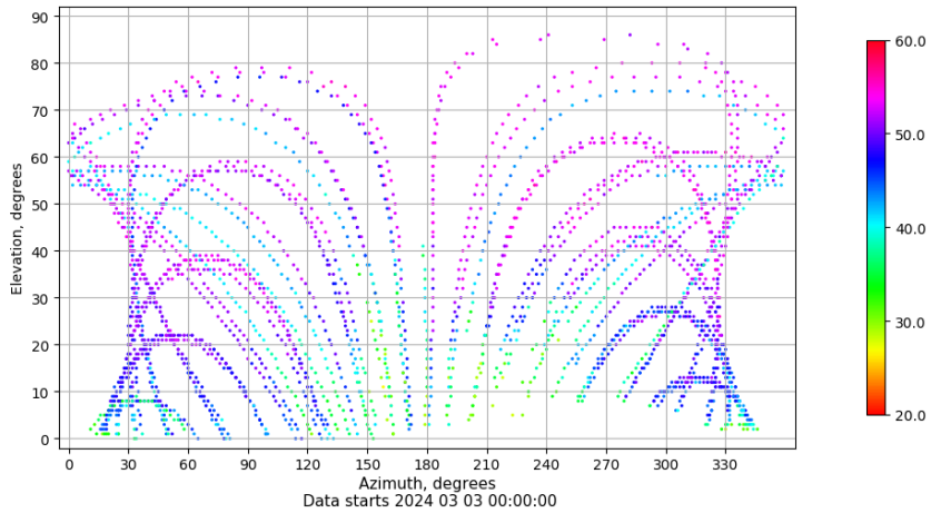
Azimuth-elevation plot for station EIVI. Signal to Noise S1C Data file EIVI00ESP_R_2024063.xtr
