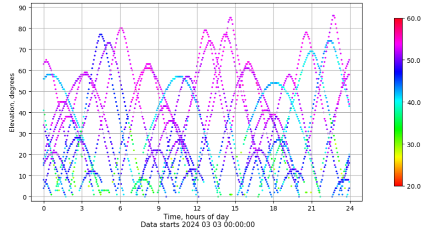
Time-elevation plot for station EIVI. Signal to Noise S1C Data file EIVI00ESP_R_2024063.xtr
