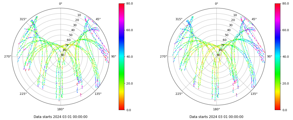
Skyplot for station EIVI. Parameter M1C Data file EIVI00ESP_R_2024061.xtr Skyplot for station EIVI. Parameter M5Q Data file EIVI00ESP_R_2024061.xtr
