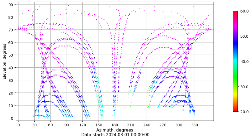
Azimuth-elevation plot for station EIVI. Signal to Noise S1C Data file EIVI00ESP_R_2024061.xtr
