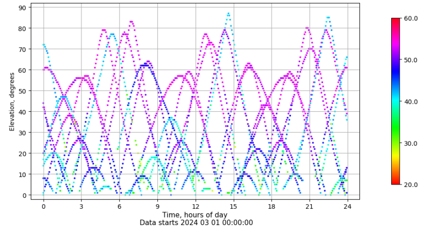
Time-elevation plot for station EIVI. Signal to Noise S1C Data file EIVI00ESP_R_2024061.xtr
