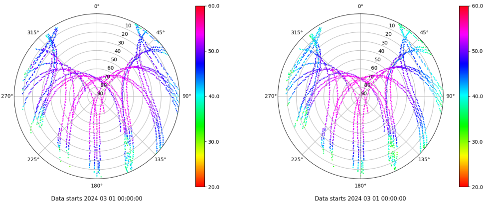
Skyplot for station EIVI. Signal to Noise S1C Data file EIVI00ESP_R_2024061.xtr Skyplot for station EIVI. Signal to Noise S5Q Data file EIVI00ESP_R_2024061.xtr
