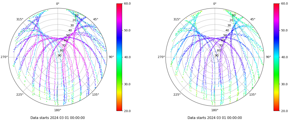
Skyplot for station EIVI. Signal to Noise S1C Data file EIVI00ESP_R_2024061.xtr Skyplot for station EIVI. Signal to Noise S2P Data file EIVI00ESP_R_2024061.xtr
