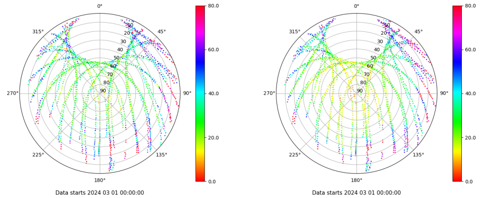
Skyplot for station EIVI. Parameter M1C Data file EIVI00ESP_R_2024061.xtr Skyplot for station EIVI. Parameter M2P Data file EIVI00ESP_R_2024061.xtr
