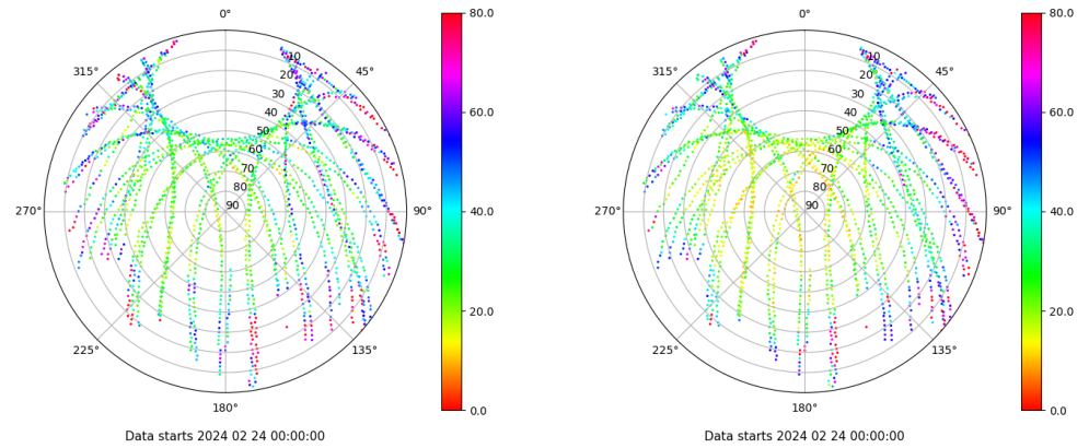
Skyplot for station EIVI. Parameter M1C Data file EIVI00ESP_R_2024055.xtr Skyplot for station EIVI. Parameter M2P Data file EIVI00ESP_R_2024055.xtr
