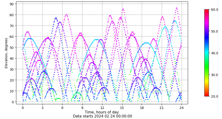
Time-elevation plot for station EIVI. Signal to Noise S1C Data file EIVI00ESP_R_2024055.xtr
