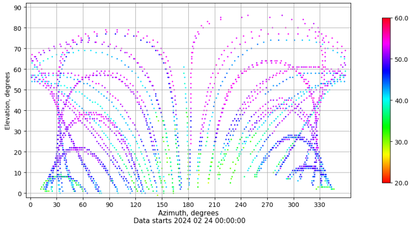
Azimuth-elevation plot for station EIVI. Signal to Noise S1C Data file EIVI00ESP_R_2024055.xtr
