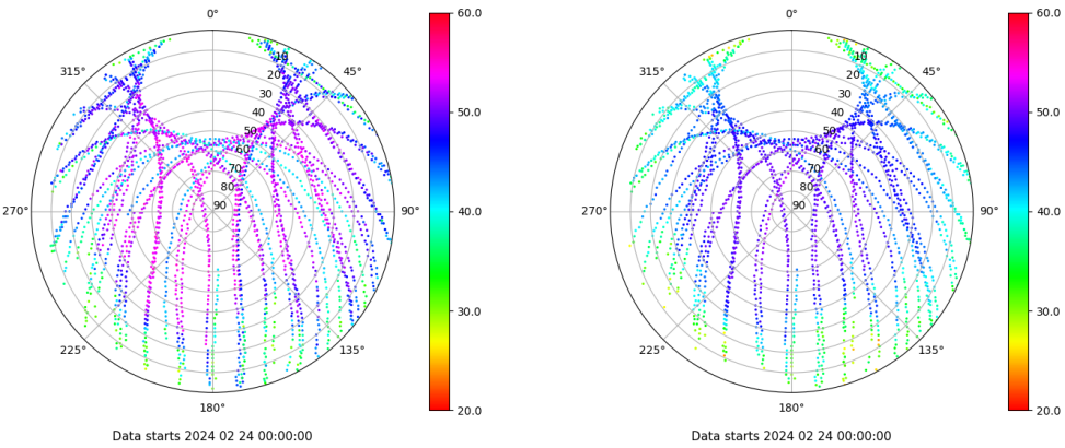
Skyplot for station EIVI. Signal to Noise S1C Data file EIVI00ESP_R_2024055.xtr Skyplot for station EIVI. Signal to Noise S2P Data file EIVI00ESP_R_2024055.xtr
