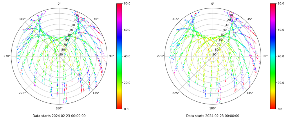
Skyplot for station EIVI. Parameter M1C Data file EIVI00ESP_R_2024054.xtr Skyplot for station EIVI. Parameter M2P Data file EIVI00ESP_R_2024054.xtr
