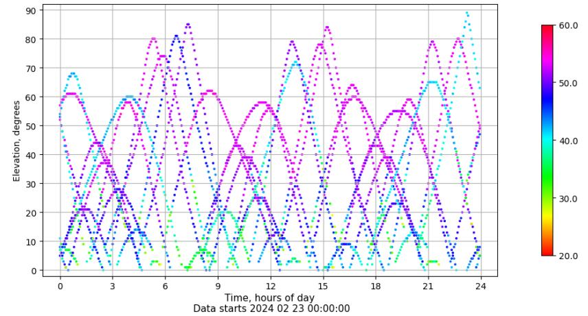
Time-elevation plot for station EIVI. Signal to Noise S1C Data file EIVI00ESP_R_2024054.xtr
