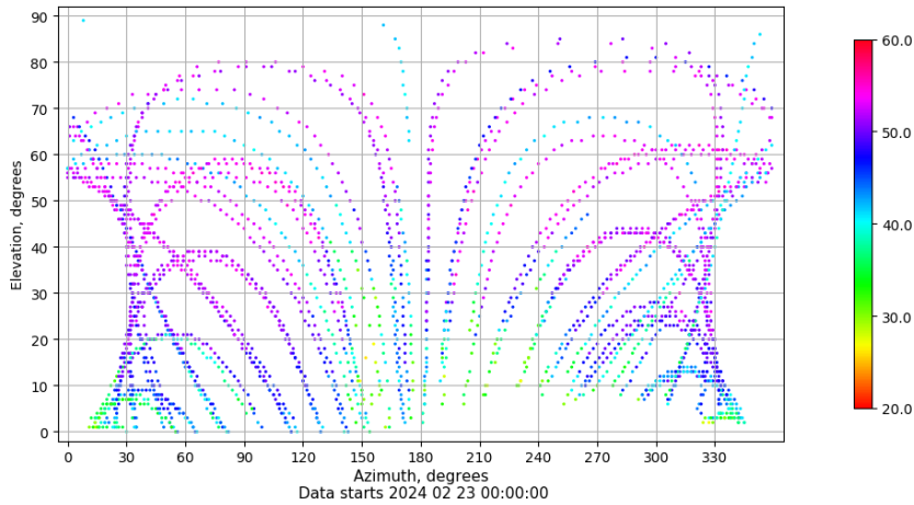
Azimuth-elevation plot for station EIVI. Signal to Noise S1C Data file EIVI00ESP_R_2024054.xtr
