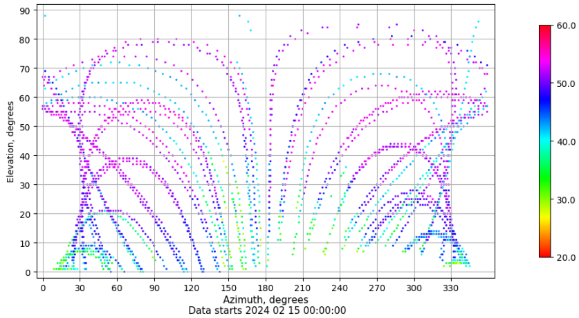
Azimuth-elevation plot for station EIVI. Signal to Noise S1C Data file EIVI00ESP_R_2024046.xtr
