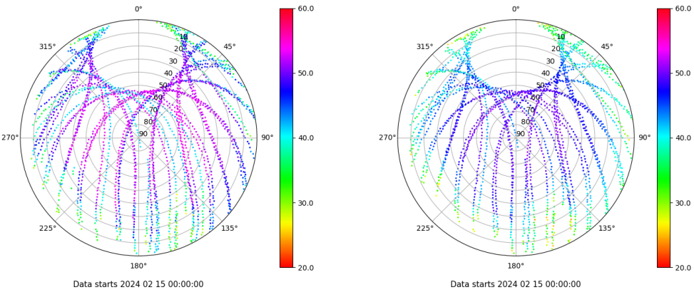
Skyplot for station EIVI. Signal to Noise S1C Data file EIVI00ESP_R_2024046.xtr Skyplot for station EIVI. Signal to Noise S2P Data file EIVI00ESP_R_2024046.xtr
