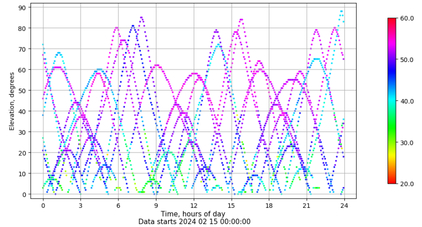
Time-elevation plot for station EIVI. Signal to Noise S1C Data file EIVI00ESP_R_2024046.xtr
